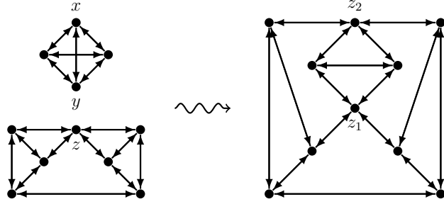
Figure 1: An example of a 4-Ore digraph obtained by an Ore-composition of two smaller 4-Ore digraphs, with replaced digon [x, y] and split vertex z .
