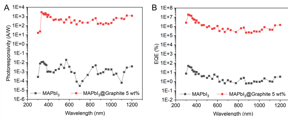
Figure 13. A) Photoresponsivity and B) effective quantum efficiency vs. wavelengths for mechanosynthesized MAPbI 3 and MAPbI 3 @Graphite 5 wt% at 10V bias
