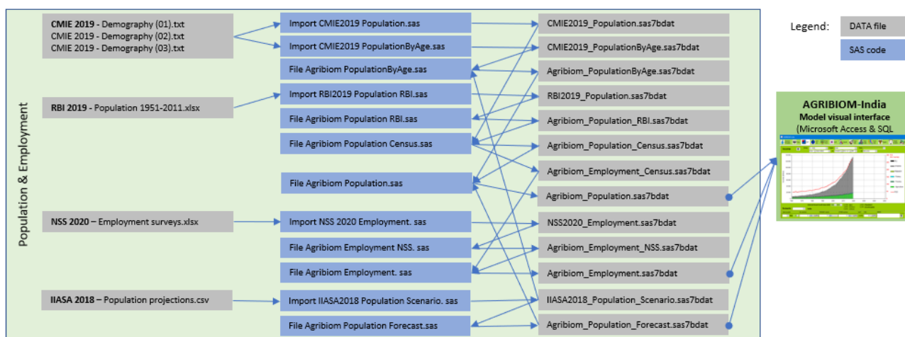
Figure 9.59. Processing chain of population and employment data in Agribiom-India
