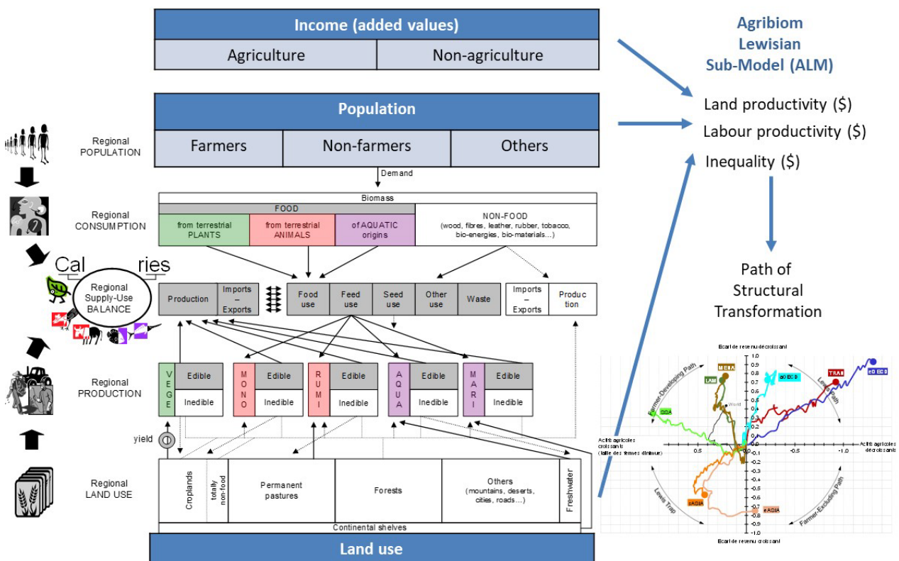
Figure 2.5. Agribiom schematic presentation
