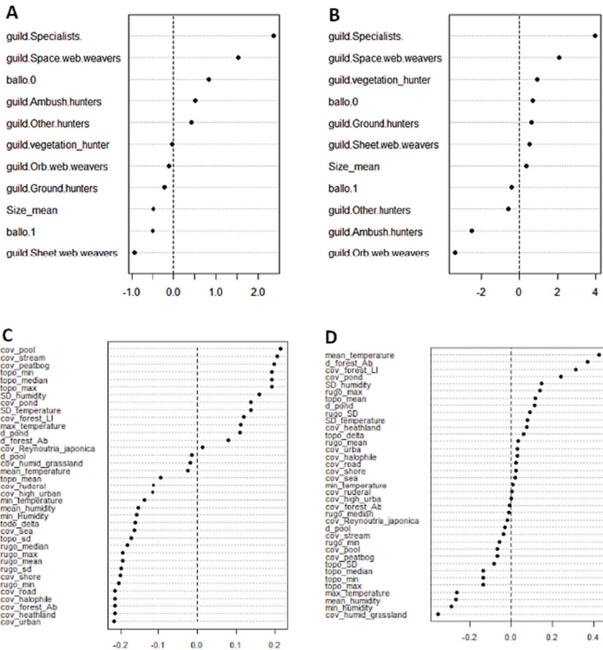
Fig. 6. The projected weight of each traits of spider’s assemblages link to the first (A) and second (B) axis and the projected weight of each environmental variable link to spider’s assemblages on the first (C) and second (D) axis. The dashed line was added to help visualize the 0.
