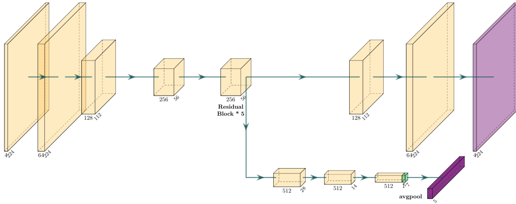
Figure 5: Architecture of the GR-ConvNet-based network used in our experiments. The input is a 224x224 RGB-D image. There are two outputs: the classification output with five classes, and the grasp output with a quality image, a width image, and two angle images, respectively as in (Morrison et al., 2018).
