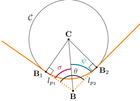
Fig. 3. Cable shape parameterization at the position of the pulley.
