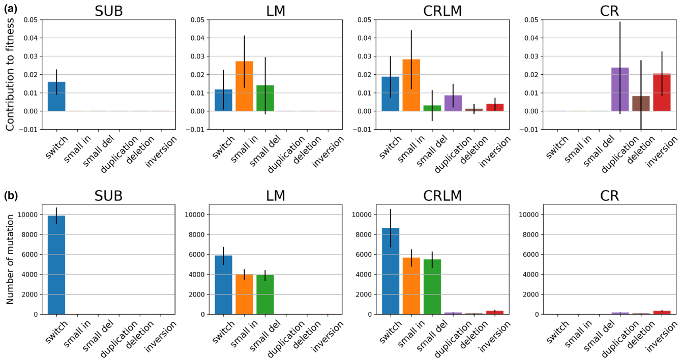
FIGURE 7 Fitness contribution and number of mutations during the evolution from WT individuals (a) Contribution of each type of mutation to the total fitness gains, measured as the sum of the change in fitness of each mutation on the line of descent of the final best individuals, starting from WT individuals. Histograms show the mean values across the 11 repetitions, and the bars show their standard deviation. Reverted mutations (mutations which effect on fitness was exactly compensated by the following one) were filtered out to reduce noise. (b) Number of fixed non-neutral and non-reverted mutations per generation for the different mutation types per million generation, normalized by the number of mutations occurring ( L \times \mu , with L the genome size), on the line of descent of the final best individuals, starting from WT individuals. Histograms show the mean values across the 11 repetitions, and the bars show their standard deviation.
