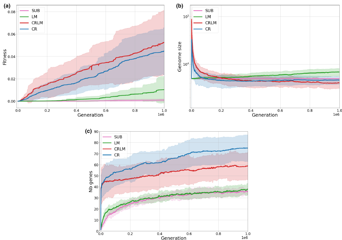
FIGURE 3 Mean variation of fitness (a), genome size (b) and gene number (c) on the line of descent of the final populations, starting from a naive individual for the four mutational scenarios. The shaded areas indicate the variability across the 11 repetitions (SD).
