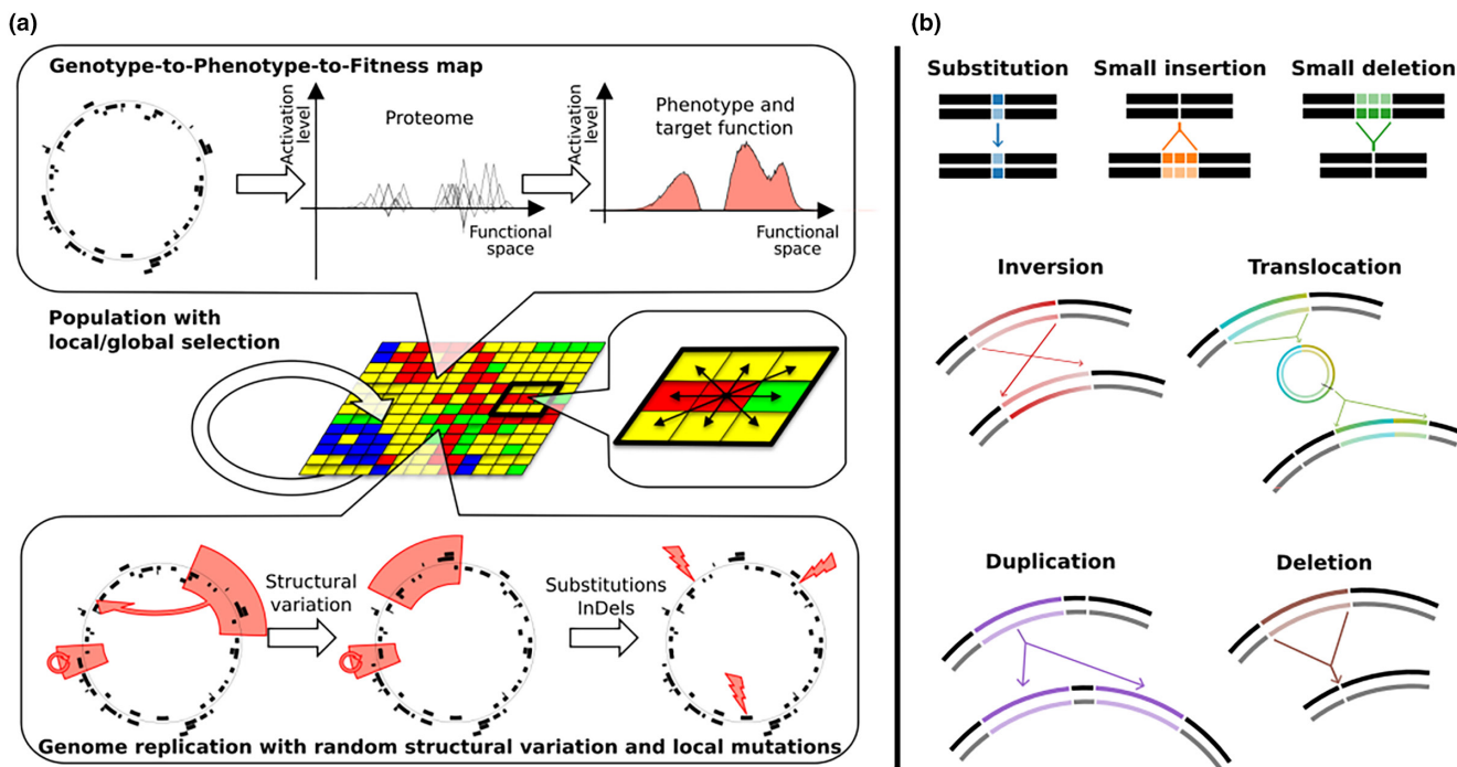
FIGURE 1 The Aevol model. The left panel (a) shows all steps of a generation in Aevol. (top) Overview of the genotype-to-phenotype map. Note that the organism shown here is a real organism evolved within Aevol for 1,000,000 generations with a typical target. It contains many Open-Reading Frames on both strands, a large proteome (the set of proteins), and it is well adapted to its environment (i.e. its phenotypic function – black curve – is very close to the target function – light red area). (middle) Population on a grid is fully renewed every generation. Example of a local selection process occurring with a 3×3 neighbourhood. (bottom) Mutation operators include chromosomal rearrangements (duplications, deletions, translocations and inversions – here a translocation and an inversion are shown) and local mutations (substitutions and InDels). These mutations are described more precisely in the right panel (b): (top) Local mutations: substitution (one base pair is mutated to another), small insertion and small deletion (a few base pairs are inserted or deleted). (middle) Balanced chromosomal rearrangements: inversion (two points are drawn and the segment in between is rotated) and translocation (a segment is excised, circularized, re-cut and inserted elsewhere in the genome). (bottom) Unbalanced chromosomal rearrangements: duplication (copy-paste of a segment in the genome) and deletion (suppression of a segment of the genome).
