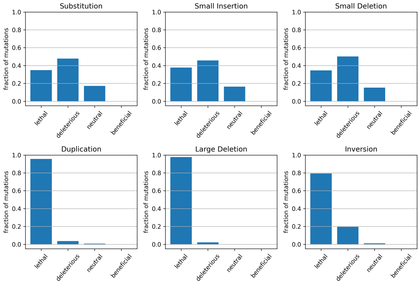
FIGURE 5 Distribution of fitness effect of the different types of mutation, on the median individual of the CRLM experiment, after 1,000,000 generations when starting from a naive individual. For each mutation type, 1,000,000 mutants were generated, except for the substitution, which were exhaustively tested. The selection coefficient is computed as s = \frac{f_{\text{mutant}}}{f_{\text{parent}}} - 1 . Lethality is defined as s < -0.999 , and neutrality as s \in [-0.001, 0.001] . The detailed Distribution of Fitness Effect (DFE) is presented in Figure S2. Interestingly, there is no advantageous substitutions available, showing that the population has reached a local fitness optimum for these mutations. However, as shown by Figure S2, a few beneficial InDels and a few beneficial segmental duplications are available, although they are not frequent enough to be visible here.
