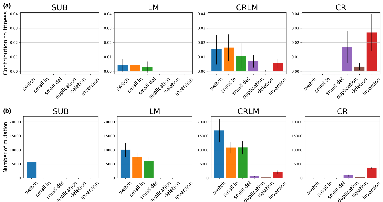
FIGURE 4 Fitness contribution and number of mutations fixed during the initial evolution from naive individuals (a) Contribution of each type of mutation to the total fitness gains, measured as the sum of the change in fitness of each mutation on the line of descent of the final best individuals, starting from naive individuals. Histograms show the mean values across the 11 repetitions, and the bars show their standard deviation. Reverted mutations (mutations which effect on fitness was exactly compensated by the following one) were filtered out to reduce noise. Fitness increase in the SUB simulations are negligible at this scale. (b) Number of non-neutral and non-reverted mutations fixed for the different mutation types and for the four conditions, normalized by the number of mutations occurring ( L \times \mu , with L the genome size), on the line of descent of the final best individuals, starting from naive individuals. Histograms show the mean values across the 11 repetitions, and the bars show their standard deviation.
