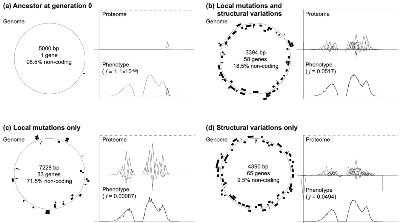
FIGURE 2 Initial ancestor (a) and examples of evolved organisms in the CRLM (b), LM (c) and CR (d) conditions after 1,000,000 generations. The organism presented in (b) corresponds to the Wild Type used for the second step of the experiments. For each organism, there is on the left a visualization of its genes localized on the genome. On the right, the proteome shows all the single proteins, and the phenotype (black curve) is their sum. The grey curve plotted in addition to the phenotype is the environmental target function, a sum of 3 Gaussian lobes (2 positives and 1 negative) – see Figure S3 . Finally, f is the absolute fitness value computed from the difference between the phenotype and the target function.
