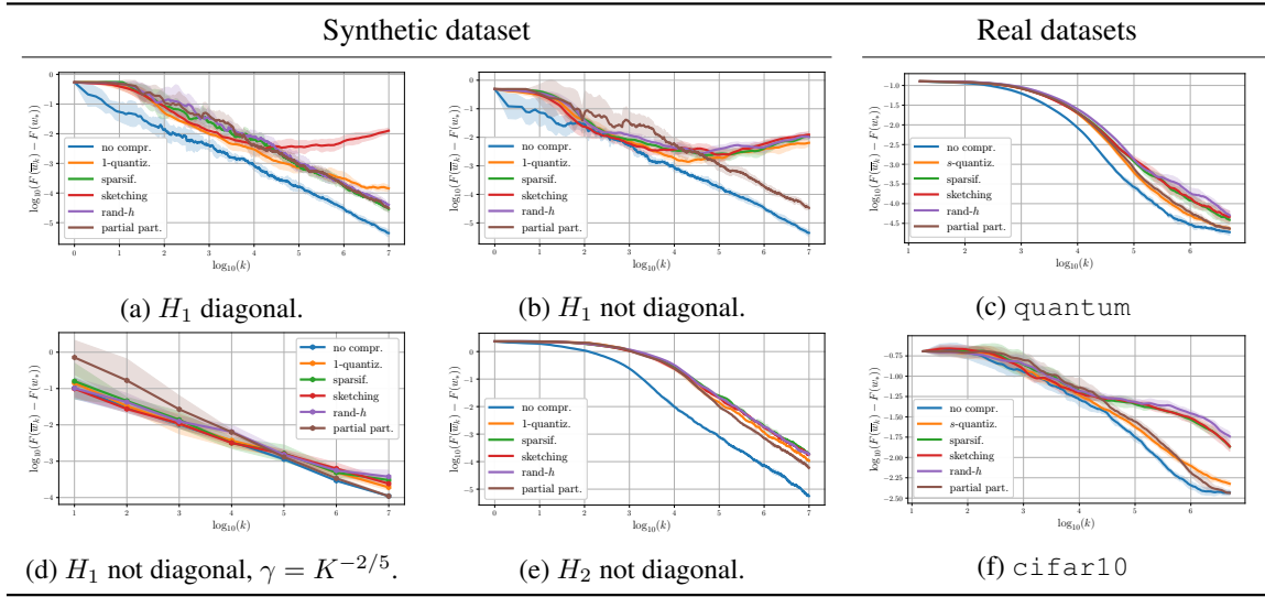
Figure 7: Logarithm excess loss of the Polyak-Ruppert iterate for a single client ( N = 1 ).
