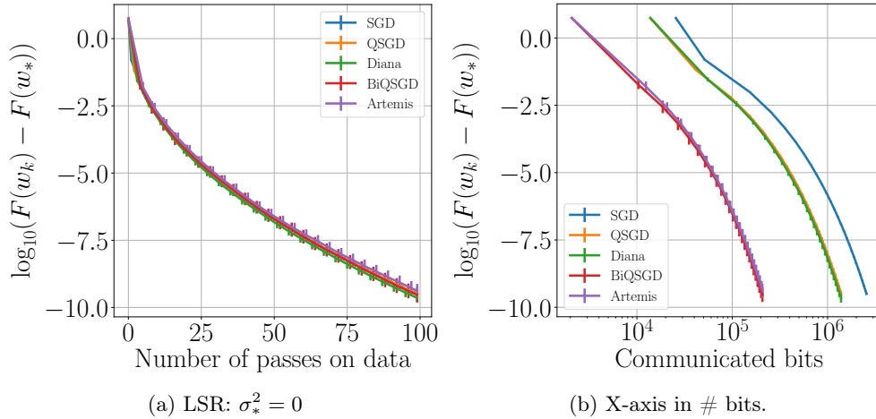
Figure S6: Synthetic dataset, Least-Square Regression without noise ( \sigma_* = 0 ). Without surprise, with i.i.d data and \sigma_* = 0 , the convergence of each algorithm is linear. Thus, in i.i.d. settings, the impact of the memory is negligible, but this will not be the case in the non-i.i.d. settings as underlined by Figure S7.
