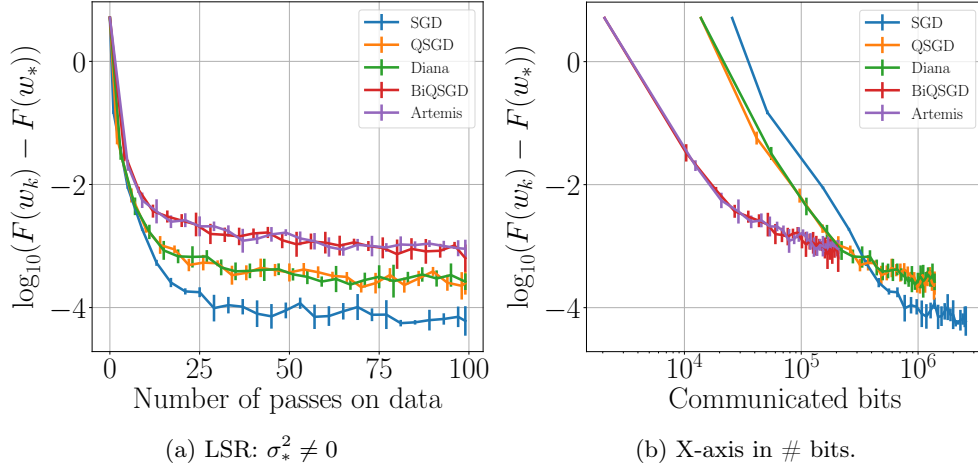
Figure S5: Synthetic dataset, Least-Square Regression with noise ( \sigma_* \neq 0 ). In a situation where data is i.i.d., the memory does not present much interest and has no impact on the convergence. Because \sigma_*^2 \neq 0 , all algorithms saturate; and saturation level is higher for double compression (Artemis, Bi-QSGD), than for simple compression (Diana, QSGD) or than for SGD. This corroborates findings in Theorem 1 and Theorem 3.
