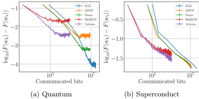
Figure 4: Real dataset (non-i.i.d.): \sigma_* \neq 0 , N = 20 workers, p = 1 , b > 1 (150 iter.). X-axis in # bits.
