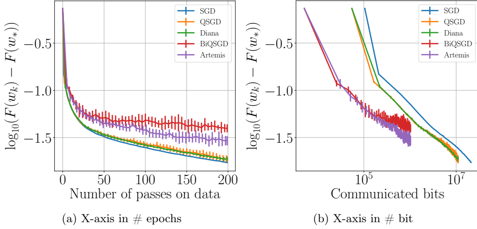
Figure S12: Superconduct . Least-squares regression, \sigma_* \neq 0 , \gamma = 1/L , b = 64 , non-i.i.d..
