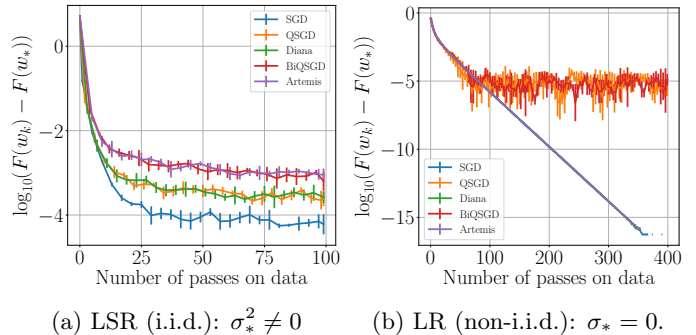
Figure 3: Left: illustration of the saturation when \sigma_* \neq 0 and data is i.i.d., right: illustration of the memory benefits when \sigma_* = 0 but with non-i.i.d. data.
