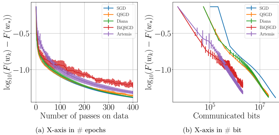
Figure S13: Superconduct . Least-squares regression, \sigma_* = 0 , \gamma = 1/L , full batch gradient descent, non-i.i.d..
