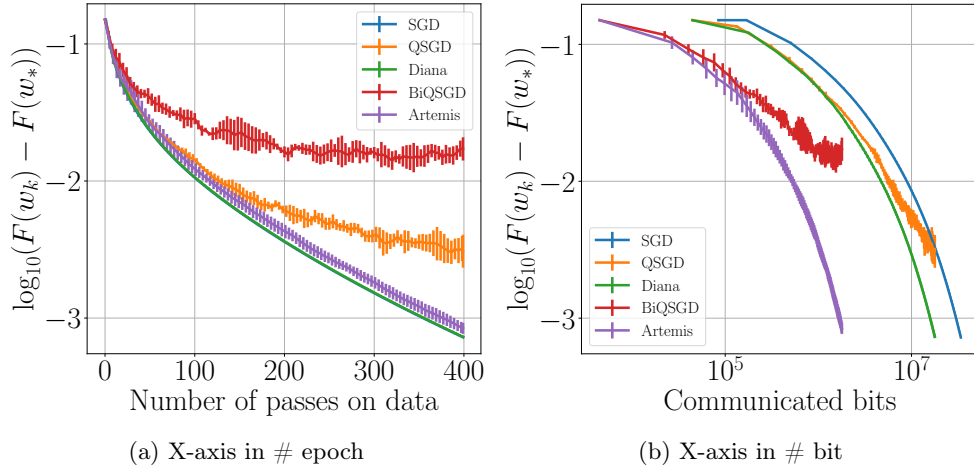
Figure S11: Quantum . Least-squares regression, \sigma_* = 0 , \gamma = 1/L , full gradient descent, non-i.i.d..
