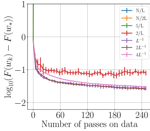
(b) Superconduct
