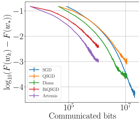
(a) Quantum
