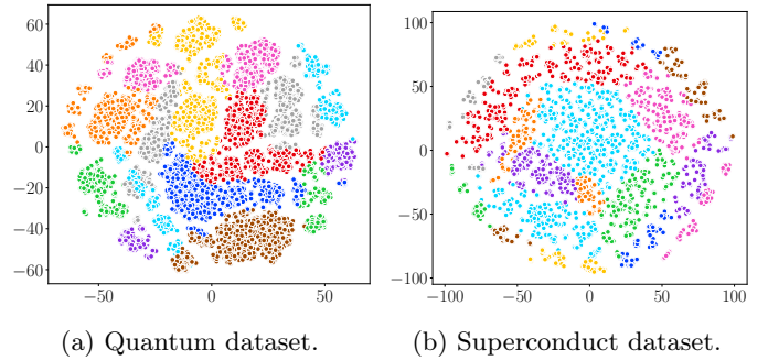
Figure 2: TSNE representations.
