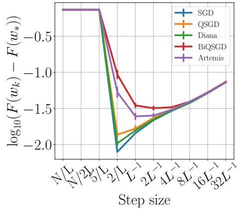
(b) Superconduct
