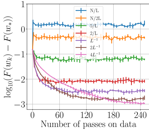
(a) Quantum
