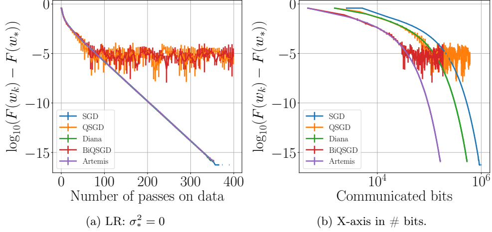
Figure S7: Synthetic dataset, Logistic Regression on non-i.i.d. data using a full batch gradient descent (to get \sigma_* = 0 ). The benefit of memory is obvious, it makes the algorithm converge linearly, while algorithms without are saturating at a higher level. This stresses the importance of using the memory in non-i.i.d. settings.
