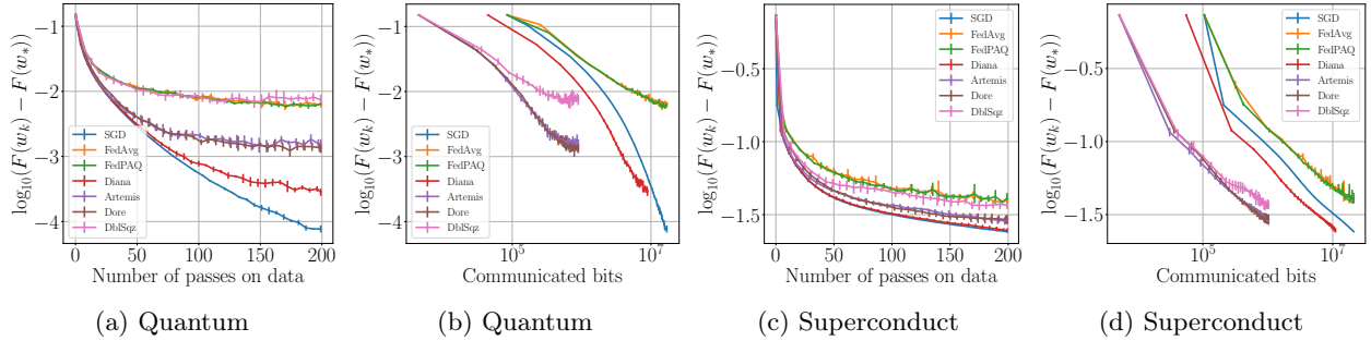
Figure S17: Artemis compared to other existing algorithms. \gamma = 1/(2L) , X-axis in # epoch or in # bits.
