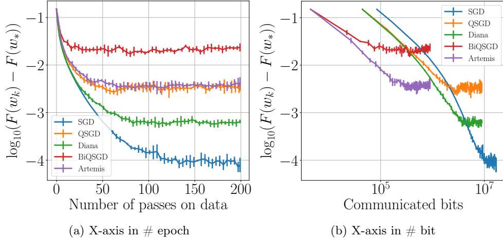
Figure S10: Quantum . Least-squares regression, \sigma_* \neq 0 , \gamma = 1/L , b = 256 , non-i.i.d..
