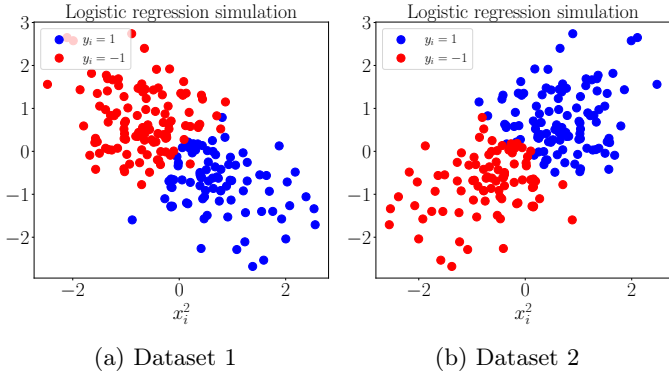
Figure 1: Data distribution for logistic regression to simulate non-i.i.d. data. Half of the device holds the first dataset, and the other half the second one.
