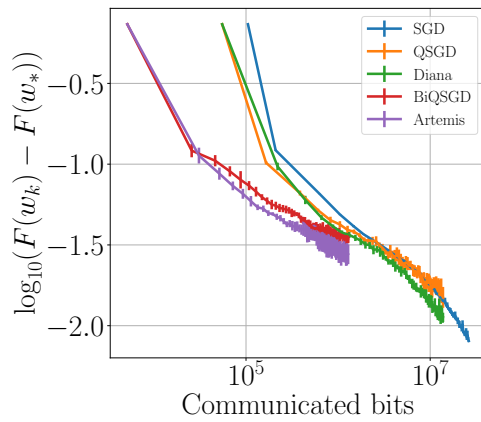
(b) Superconduct
