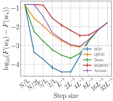
(a) Quantum
