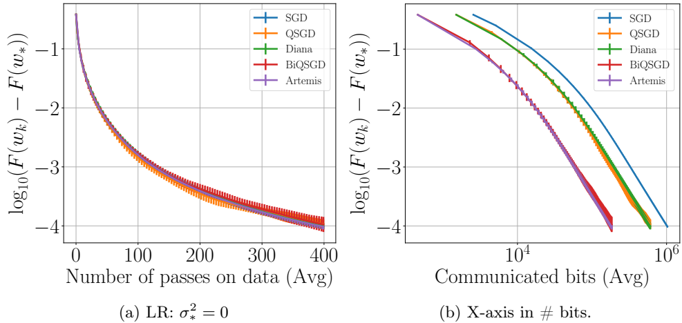
Figure S8: Polyak-Ruppert averaging, synthetic dataset. Logistic regression on non-i.i.d. data using a full batch gradient descent (to get \sigma_* = 0 ) and a Polyak-Ruppert averaging. The convergence is sublinear as predicted by Theorem 2 because \sigma_* = 0 .
