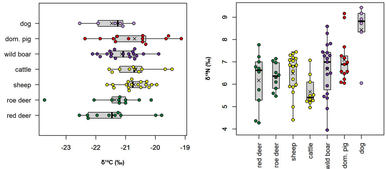
Fig 3. Stable carbon ( \delta^{13}\text{C} ) and nitrogen ( \delta^{15}\text{N} ) isotope ratio results for mammal bone collagen from the Starčevo phase at Alsónyék, subsite 5603/1. This figure shows the same data as in Fig 2, but visualised as boxplots. The line in the boxplot indicates the median, and the cross the mean. Whisker boundaries were chosen as 1.5 \times interquartile range. Fish and foxes were excluded due to low sample numbers.
