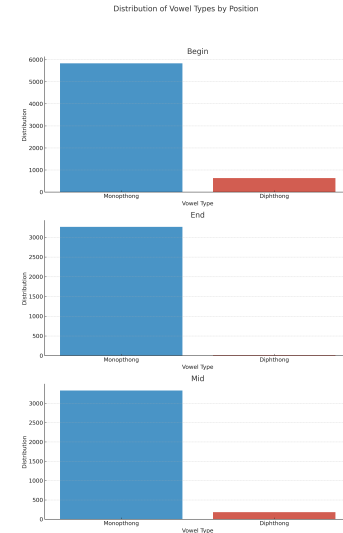
Fig. 2. Distribution of Vowel Types by Position
