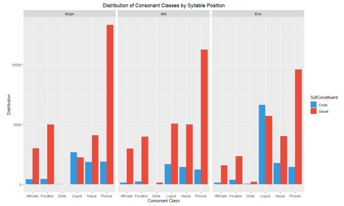
Fig. 1. Distribution of Consonant Classes by Syllable Positions
