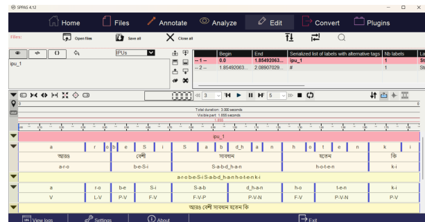
Fig. 3. SPPAS output example of a Bengali sentence
