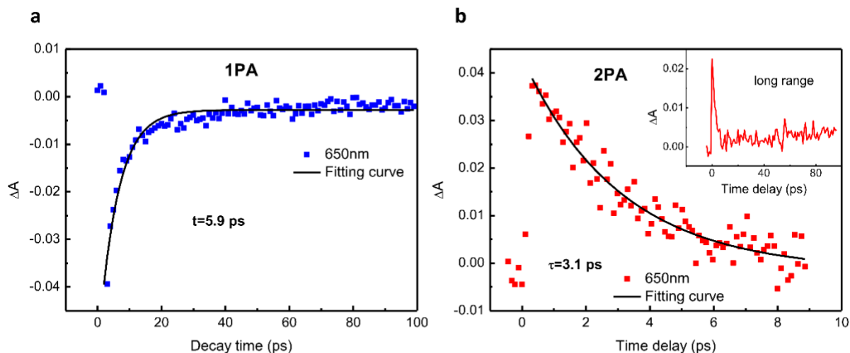
Figure S1. The dynamics of the strongly coupled TDBC molecules at 1PA and 2PA excitations. (a) Temporal evolution of the |P\rangle emission at 650 nm when excited at 555 nm (1PA) under a fluence of 50 \mu\text{J}/\text{cm}^2 . (b) Dynamics of the populated |P\rangle at 650 nm when pumped at 1110 nm (2PA) under a fluence of 5 \text{ mJ}/\text{cm}^2 . Inset to (b), long range measurements for the dynamics of the 2PA-induced |P\rangle .
