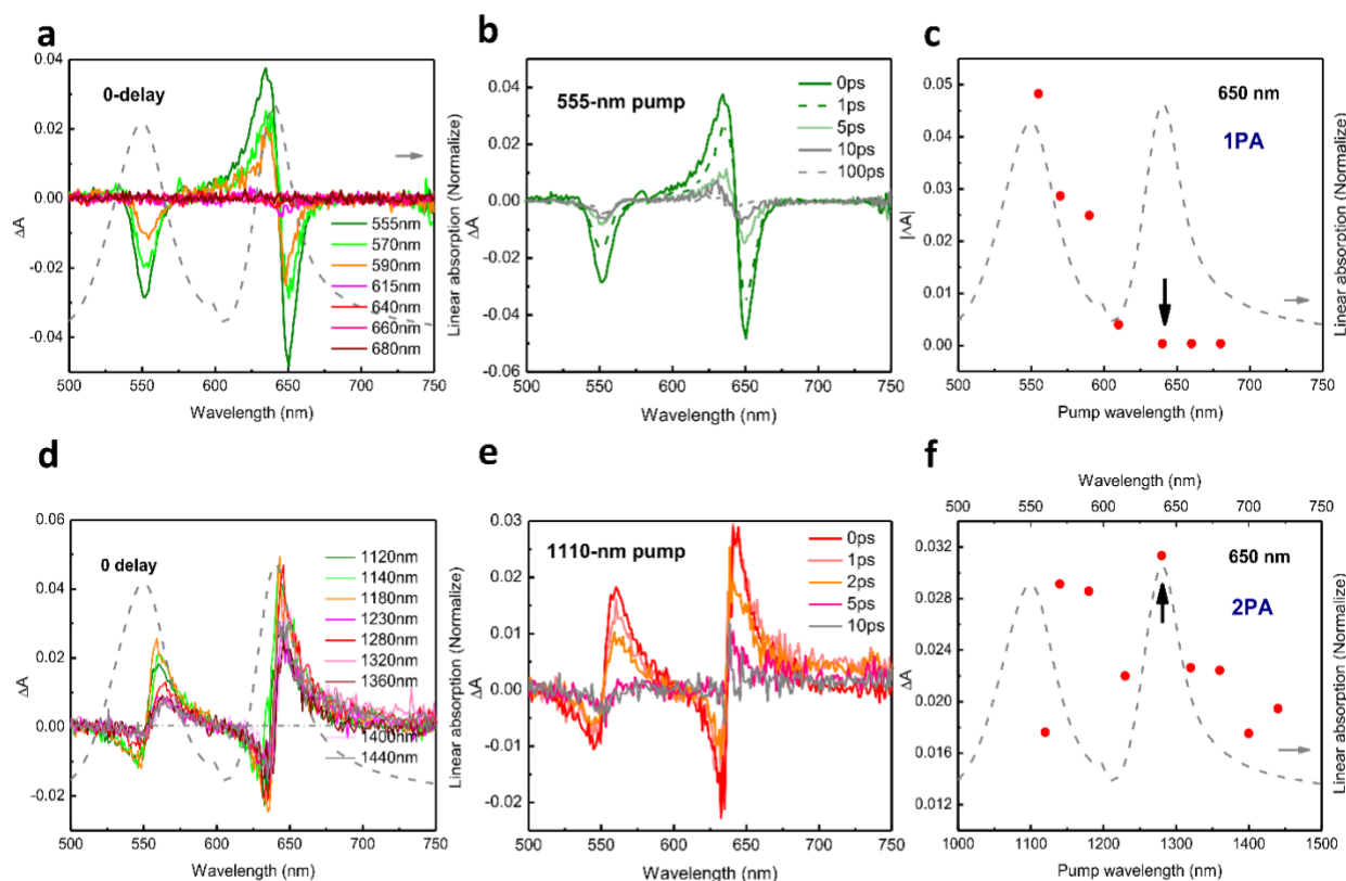
Figure 3. Nonlinear optical spectroscopy of TDBC J-aggregate under ESC. (a, d) Transient absorption spectra at zero delay, (b, e) temporal evolution of the transient spectra at typical pumping wavelengths, (c, f) action spectra recorded near |P\rangle resonance (650 nm) under 1PA excitation (upper panel (a-c), 50 \mu\text{J}/\text{cm}^2 ) and 2PA excitation (lower panel (e-f), 5 \text{ mJ}/\text{cm}^2 ). Both the pump and probe beams are kept near normal incidence. The black arrows in (c) and (f) denote \lambda_{|P\rangle} and 2\lambda_{|P\rangle} , respectively, for the TDBC cavity. The dashed grey curves, which denote linear absorption spectrum of the ESC cavity for TDBC J-aggregate, are references for transient and action spectra in (a, c, d, f).
