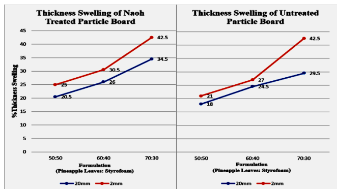
Figure 5. Effects of particle size, formulation & NaOH Treatment on the thickness swelling of the particleboard for 24 hrs.
