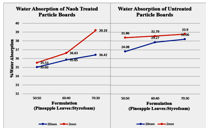
Figure 4. Effects of particle size, formulation & NaOH Treatment on the water absorption of the particleboard (24 hrs.)
