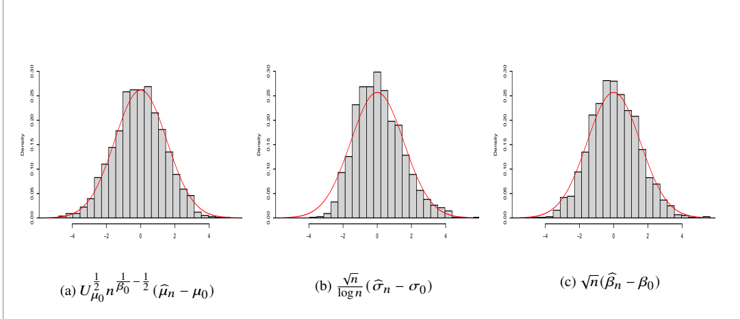
Figure 3: Distributions of the re-scaled errors of the maximum likelihood estimation (MLE) and comparison with their theoretical Gaussian limits
