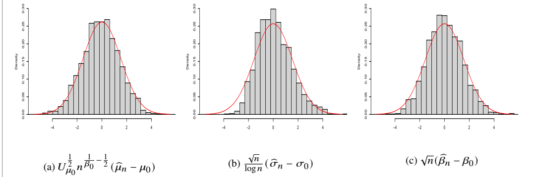
Figure 3: Distributions of the re-scaled errors of the maximum likelihood estimation (MLE) and comparison with their theoretical Gaussian limits
