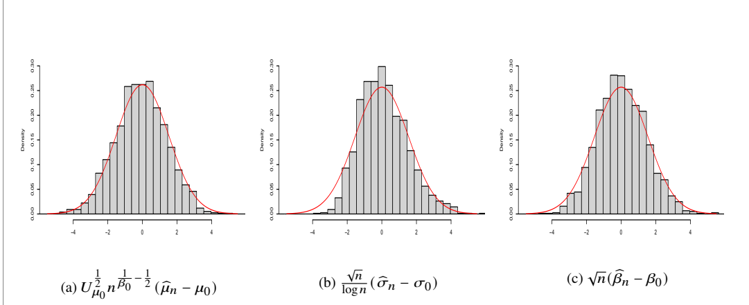
Figure 3: Distributions of the re-scaled errors of the maximum likelihood estimation (MLE) and comparison with their theoretical Gaussian limits
