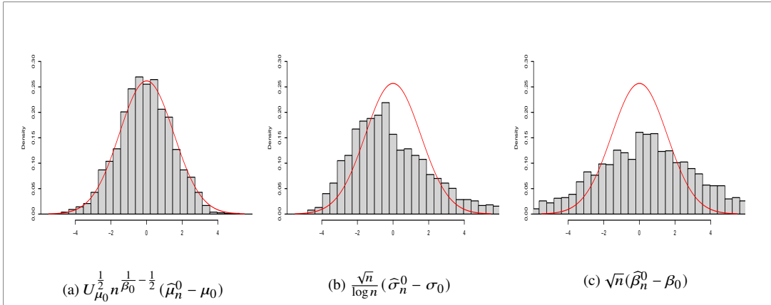
Figure 1: Distributions of the re-scaled errors of moment estimation (ME) and comparison with the asymptotic normal distribution with efficient variance given by (4.3)
