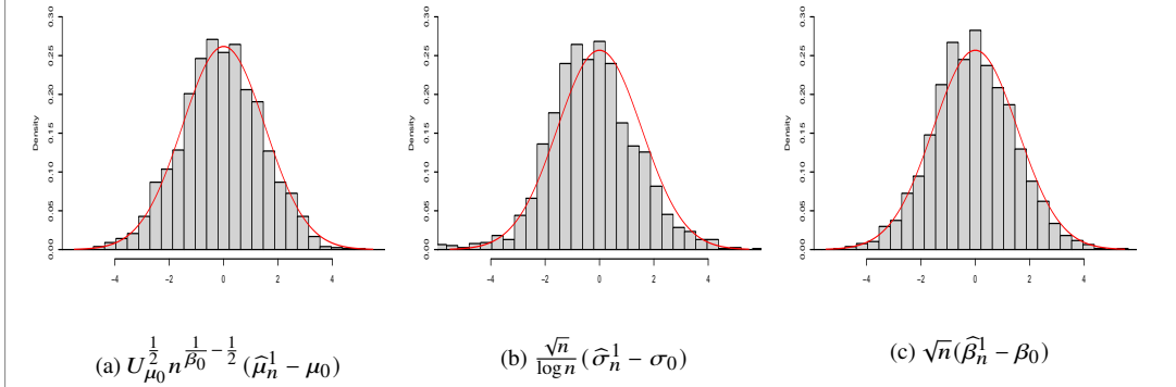
Figure 2: Distributions of the re-scaled errors of one-step estimation (OS) and comparison with their theoretical Gaussian limits
