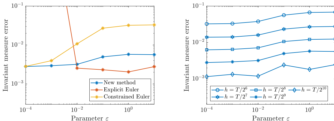
Figure 1: Error for sampling the invariant measure of penalized Langevin dynamics on a torus in \mathbb{R}^3 of the uniform discretization (2.2) and the Euler integrators (1.5) and (1.6) for different values of \varepsilon with h = 2^{-9}T (left), and error curves versus \varepsilon of the uniformly accurate method for different timesteps h = 2^{-i}T and i = 6, \dots, 10 (right), with the final time T = 10 , the maps f(x) = -25(x_1 - R + r, x_2, x_3) , \phi(x) = |x|^2 , and M = 10^7 trajectories.
