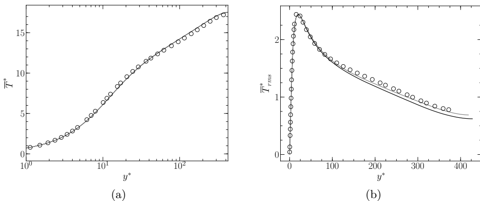
Figure 4: Downstream equilibrium state. Profiles of mean (a) and r.m.s. (b) temperature: — present results with 2\pi\delta -long bi-periodic channel flow (gray) and at x/\delta \approx 18\pi ; \circ results from Kawamura et al. (1999).
