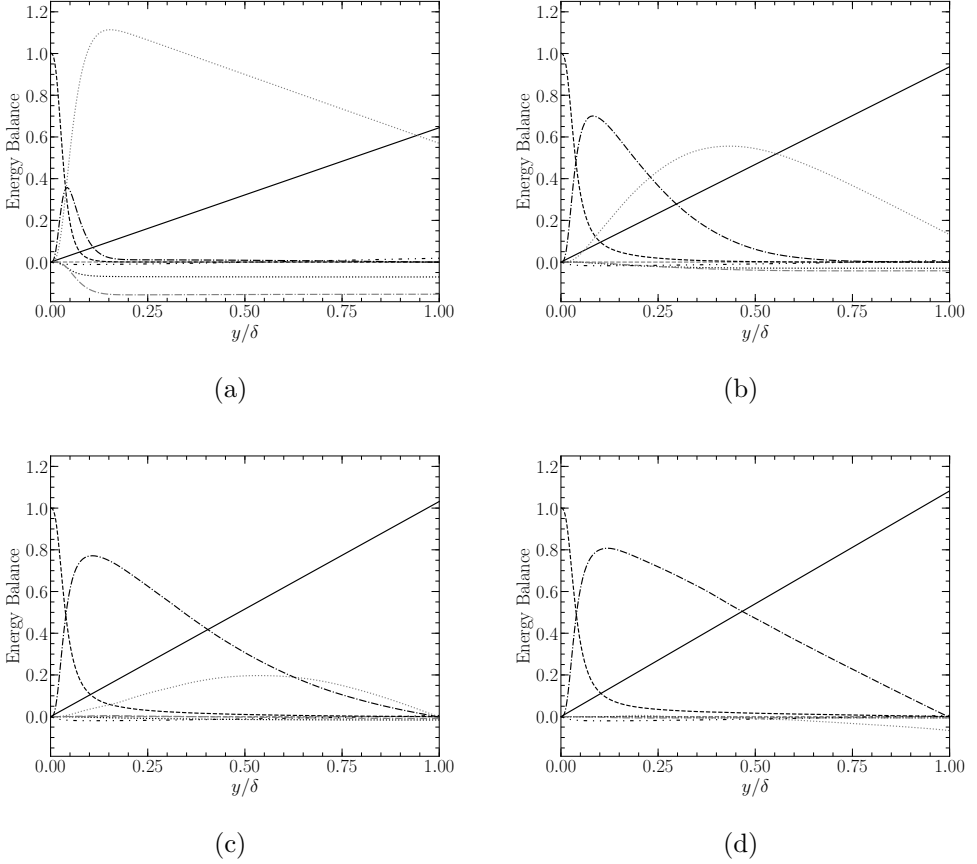
Figure 15: Energy flux balance at x/\delta = 0.73 (a), 2\pi (b), 5.7\pi (c) and 16.5\pi (d): — source term; - - - streamwise (gray) and wall-normal (black) conductive fluxes; ···· streamwise (gray) and wall-normal (black) convective fluxes; - · - · streamwise (gray) and wall-normal (black) turbulent fluxes; - · - - compressibility effects.
