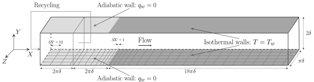
Figure 1: Computational domain of the present study.
