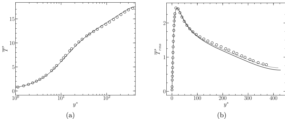
Figure 4: Downstream equilibrium state. Profiles of mean (a) and r.m.s. (b) temperature: — present results with 2\pi\delta -long bi-periodic channel flow (gray) and at x/\delta \approx 18\pi ; ○ results from Kawamura et al. (1999).
