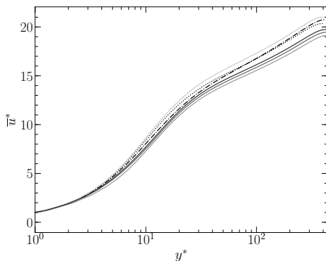
Figure 9: Mean streamwise velocity profile for different x/\delta in semi-local scaling: — present results at x/\delta = -0.06, 0.015, 0.09, 0.18 (from lightest to darkest respectively); \cdots equilibrium profile of §3.1; -\cdot-\cdot- equilibrium profile of §3.2.
