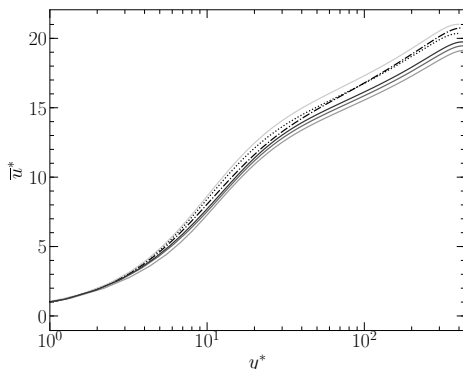
Figure 9: Mean streamwise velocity profile for different x/\delta in semi-local scaling: — present results at x/\delta = -0.06, 0.015, 0.09, 0.18 (from lightest to darkest respectively); ····· equilibrium profile of §3.1; - - - - equilibrium profile of §3.2.
