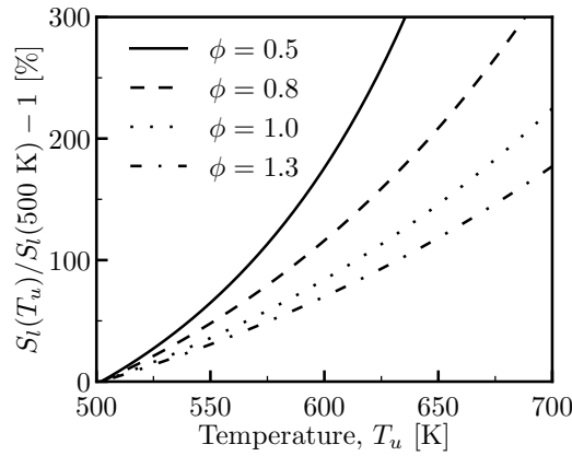
Figure 11: Temperature sensitivity of adiabatic flame speeds for different equivalence ratios at p = 5 \text{ atm} , y_{\text{H}_2\text{O}}^0 = 0.3 and with L = 20 \text{ cm} .
