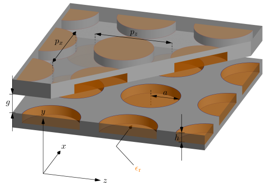
Fig. 1. GS holey PPW with circular holes. The two holey structures are off-shifted of half a period in the two periodicity directions (glide symmetry). The holes depth is h and a material having dielectric constant \epsilon_{r2} fill them. The wave propagates in the gap between the metasurfaces, filled with air ( \epsilon_{r1} = 1 not shown).
