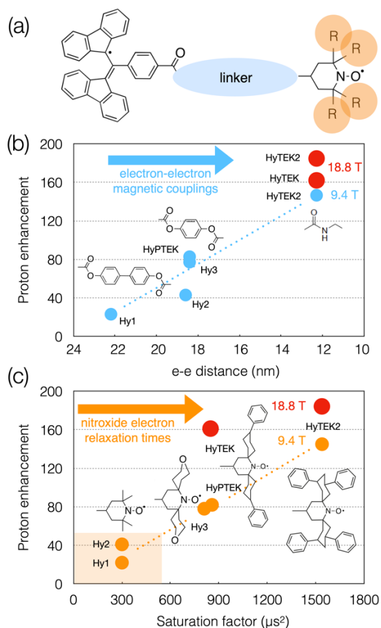
Figure 8: (a) Schematic structure of BDPA-nitroxide hybrid radicals. (b) and (c): Plots showing the evolution of the enhancement factor with electron-electron distance (b) and saturation factor (c) in the HyTEK series. The blue and orange dots correspond to data acquired at 9.4 T, while the red dots are values measured at 18.8 T. Adapted from reference 113.
