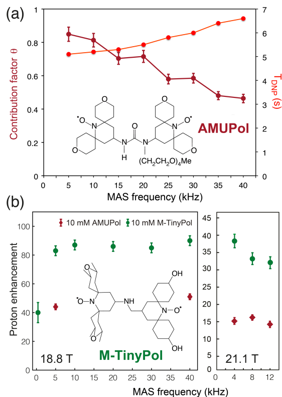
Figure 6: (a) Contribution and build-up times for a 10 mM AMUPol solution in d_8 -glycerol/ D_2O / H_2O (60/30/10, v/v/v) at 18.8 T as a function of MAS rate. The structure of AMUPol is shown. Adapted from reference 91 with permission from RSC Publishing, copyright 2016. (b) Enhancement factors of M-TinyPol at 10 mM measured in bulk solution of d_8 -glycerol/ D_2O / H_2O (60/30/10, v/v/v) at 18.8 T and 21.1 T as a function of MAS frequency. Adapted from reference 94 with permission from RSC Publishing, copyright 2020.
