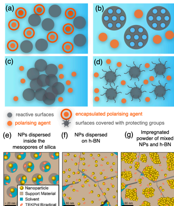
Figure 12. (a-d) Schematic views of strategies implemented for DNP SENS on reactive surfaces, in non-porous (a, c and d) or porous (b) materials. (a) the reactive surfaces are represented as grey balls while the orange spheres represent the radical (e-g) General schemes of sample preparation methods for DNP SENS on nanoparticles and quantum dots. (e) The particles (in yellow) are dispersed inside the mesopores of silica or (f) on hexagonal boron nitride (h-BN). (g) A powdered mixture of the particles and the h-BN support is impregnated with the radical solution, which increases the concentration of NPs in the formulated sample. (e-g): adapted with permission from reference 165. The sample preparation schemes (a-g) are not drawn to scale.
