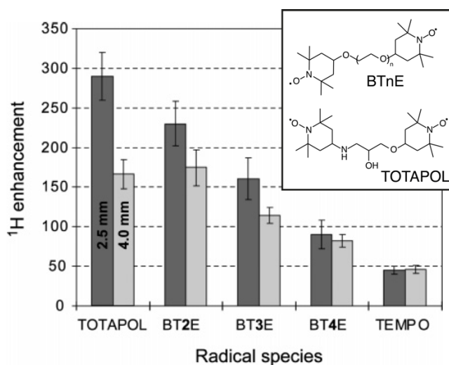
Figure 2: Structures of BTnE and TOTAPOL radicals and measured DNP enhancements at 5 T and 90 K. Reproduced and adapted from reference 56 with permission from American Chemical Society, copyright 2006.
