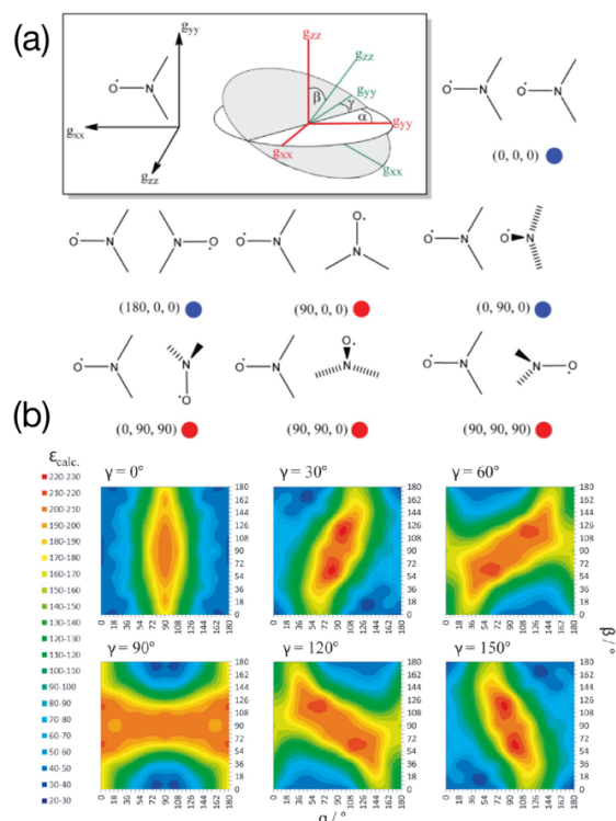
Figure 3: (a) The orientation of the g -tensor in the nitroxide molecular frame as well as the coordinate frame defining the three Euler angles. Different biradical orientations are outlined and their corresponding Euler angle values are listed. Red circles indicate favorable orientations while blue circles indicate unfavorable orientations. (b) Calculated enhancements for six ensembles of (\alpha, \beta, \gamma) Euler angles between the g -tensors. Reproduced and adapted from reference 63 with permission from John Wiley & Sons, copyright 2017.
