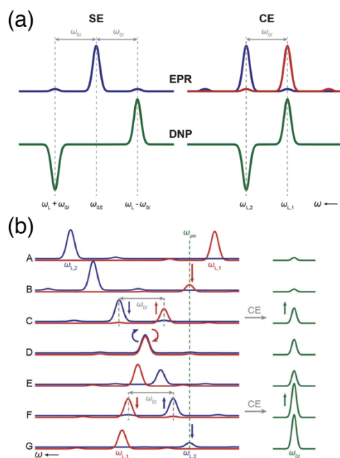
Figure 1: (a) Schematic EPR and DNP field profiles for SE and CE showing the separation between the positive and negative maximum enhancements. The satellite transitions visible in the EPR spectra correspond to forbidden ZQ and DQ transitions. (b) The Larmor frequency of the two electrons (in red and blue) is modulated during magic angle spinning (from A to G). Several rotor events are taking place, such as electron-microwave frequency crossing (B and G), cross-effect (C and F) or electron-electron frequency crossing (D), that result in polarization transfers to the nucleus (in green). Reproduced from reference 22 with permission from the RSC publishing, copyright 2016.
