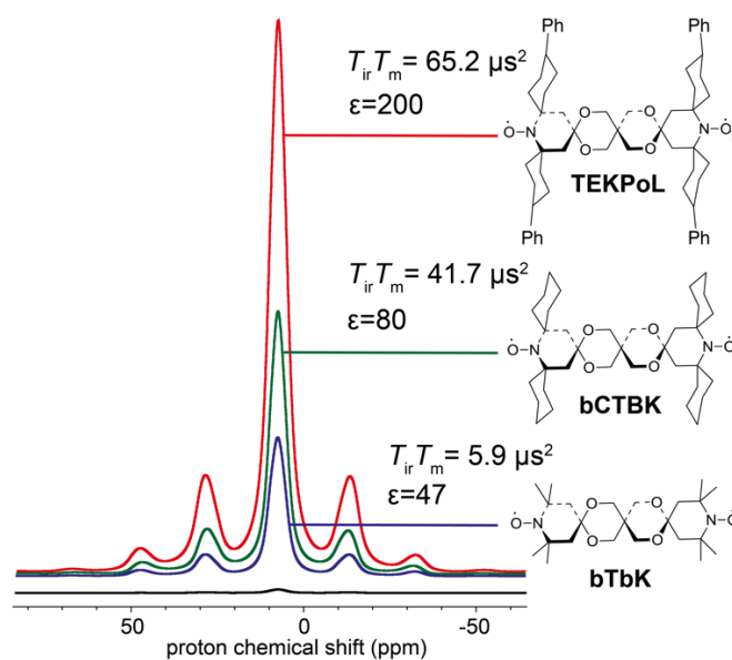
Figure 4: Proton enhancement and saturation factors measured for 16 mM bTbK, bCTbK and TEKPOL in frozen solution of TCE at 100 K. The black spectrum is the microwave off signal. Adapted from reference 70.
