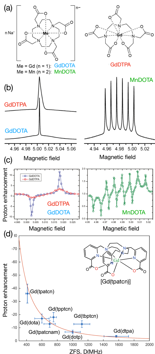
Figure 9: Structures (a), EPR profiles (b) and Zeeman field profiles (c) recorded under MAS DNP conditions at 5 T for Gd(DOTA) in blue and Gd(DTPA). Reproduced from reference 122 with permission from American Chemical Society, copyright 2011. (d) Proton DNP enhancement at 9.4 T for 4 mM solutions in DNP juice of seven different Gd(III) complexes as a function of their axial zero field splitting parameter D. The red curve is a fit to the theoretical inverse quadratic relationship. Reproduced from reference 127 with permission from American Chemical Society, copyright 2022.
