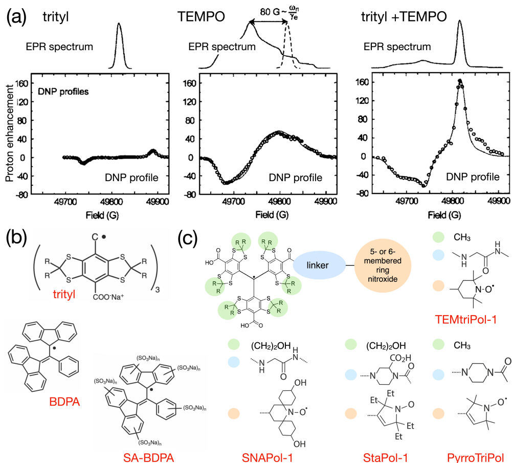
Figure 7: (a) EPR spectra and Zeeman field profiles recorded at 5 T and 90 K for trityl, 4-hydroxy-TEMPO and a 1:1 mixture of these radicals. Reproduced and adapted from reference 98 with permission from American Chemical Society, copyright 2007. (b) Molecular structure of trityl, BDPA and the water-soluble sulfonated BDPA. (c) Schematic structure of trityl-nitroxide hybrid radicals, and substituents for TEMTriPol-1 103 , SNAPol-1, 104 StaPol 105 and PyrroTriPol. 106
