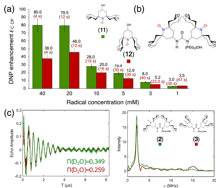
Figure 5: (a) Proton MAS DNP enhancements measured via ^1\text{H} - ^{13}\text{C} CP for the monoradicals O-MbPyTol (in green) and C-MbPyTol (in red) in \text{DMSO-}d_6\text{:D}_2\text{O:H}_2\text{O} (60:30:10 v/v/v) at different radical concentrations at 9.4 T and 100 K. The enhancement value is indicated in black above the bar. The build-up time of the solvent ^1\text{H} signals is given in parentheses. (b) Structure of the HydrOPol. (c) Three-pulse ESEEM time-domain data and the corresponding magnitude spectra (obtained after Fourier Transform of the normalized nuclear modulation function) for O-MAMUPOL (in green) and C-MAMUPOL (in red) in glycerol- d_3\text{:D}_2\text{O:H}_2\text{O} (60:30:10 v/v/v) at 50 K and 200 \mu\text{M} . The solvent accessibility parameter \Pi(D_2O) , obtained from the modulation depth defined as the peak-to-peak distance between the first maximum and the first minimum in the deuterium modulation, 90 is always larger for the open form. Reproduced from reference 90 with permission from American Chemical Society, copyright 2020.
