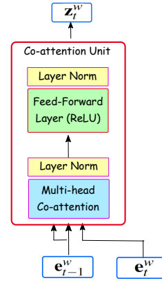
Fig. 3. Co-attention unit
