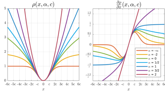
Fig. 4. The general robust loss function proposed in [4].
