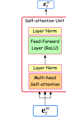
Fig. 2. Self-attention unit
