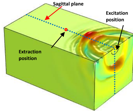
Figure 4: Simulation results : displacement at instant t_i=3.7\mu s .
