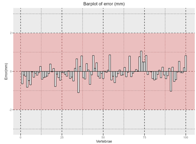
Fig. 4: \Delta_{depth} of the 100 lamb spinous processes drilling
