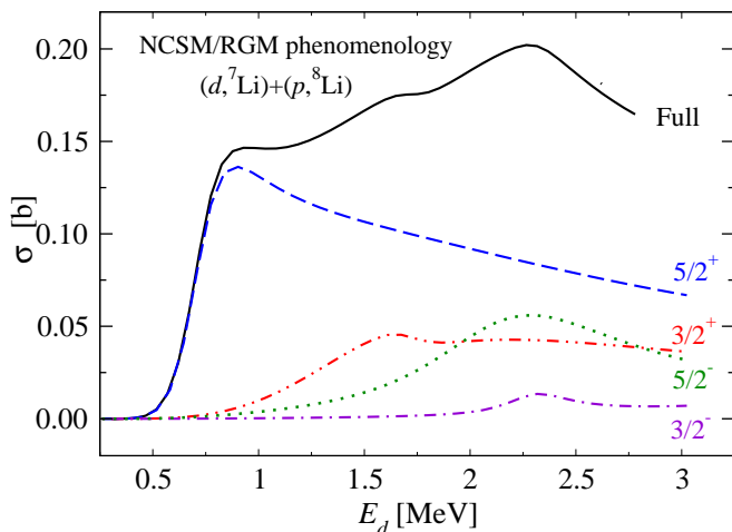
FIG. 9. Contribution of dominant J^\pi ( T = \frac{1}{2} ) partial waves to the NCSM/RGM phenomenology total cross section (solid line) shown in Fig. 8.
