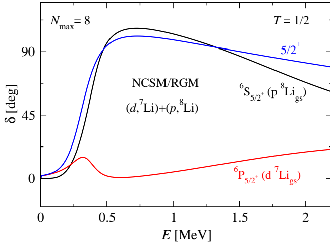
FIG. 3. Eigenphase shifts for the J^\pi T = \frac{5}{2}^+ \frac{1}{2} partial wave (solid blue line) compared to the d - {}^7\text{Li} (solid red line) and p - {}^8\text{Li} (solid black line) elastic phase shifts contributing to the same partial wave through a P - and S -wave respectively. All results were obtained within the coupled (d, {}^7\text{Li})+(p, {}^8\text{Li}) NCSM/RGM basis, and are plotted as a function of the relative kinetic energy in the c.m. frame with respect to the p+{}^8\text{Li} threshold.
