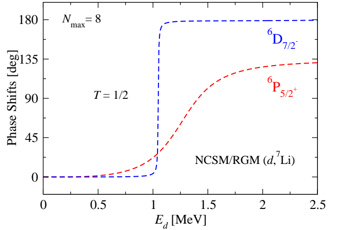
FIG. 6. Resonant d-{}^7\text{Li} {}^6D_{7/2} and {}^6P_{5/2} phase shifts as functions of the kinetic energy of the deuteron projectile in the laboratory frame, calculated within the (d,{}^7\text{Li}) NCSM/RGM basis. The SRG- N^3\text{LO} NN potential with \Lambda=2.02 \text{ fm}^{-1} , the N_{\text{max}}=8 basis size, and the HO frequency of \hbar\Omega=20 \text{ MeV} were used.
