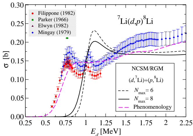
FIG. 8. {}^7\text{Li}(d,p){}^8\text{Li} integrated cross section for deuteron laboratory energies up to 2.25 MeV computed within the NCSM/RGM approach at N_{\text{max}} = 6 (thin-dashed line) and 8 (solid line) compared to the experimental data from Refs. [23, 25, 26, 45] (symbols). Also shown as a thick dashed magenta line is the result of the NCSM/RGM phenomenology approach (see text for details).
