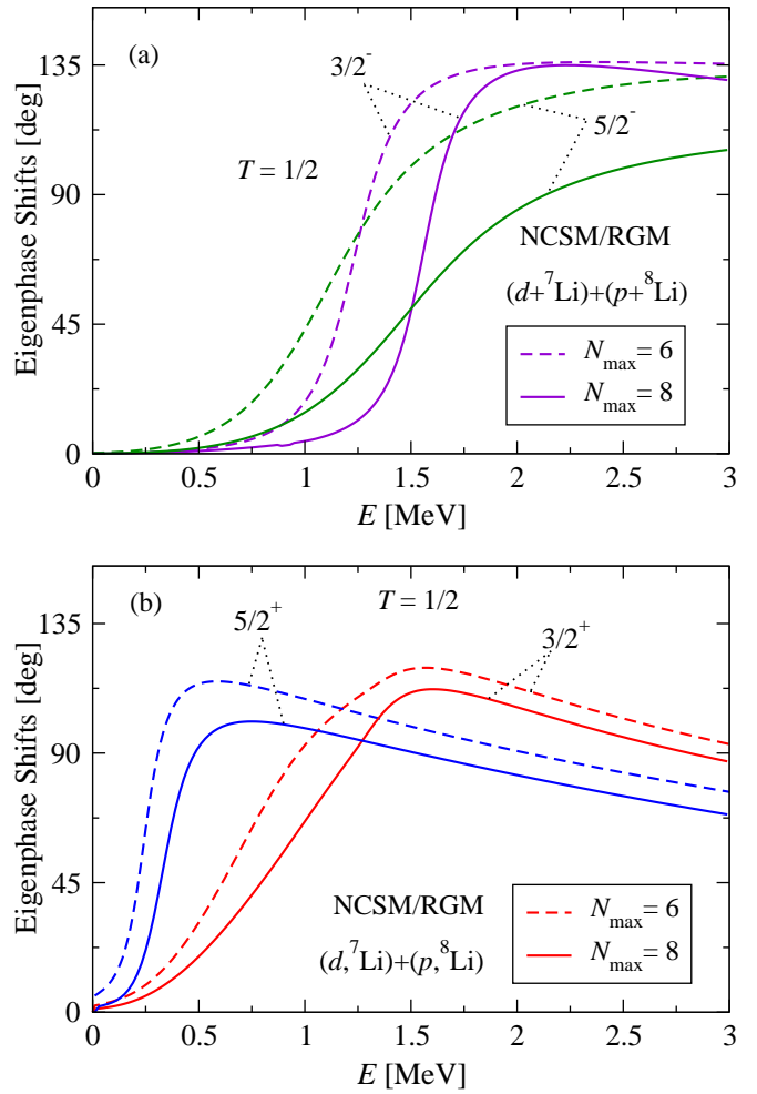
FIG. 2. Calculated (a) negative and (b) positive-parity eigenphase shifts within the coupled (d, {}^7\text{Li})+(p, {}^8\text{Li}) NCSM/RGM basis, as a function of the relative kinetic energy in the c.m. frame with respect to the p+{}^8\text{Li} threshold. The SRG- N^3\text{LO} NN potential with \Lambda=2.02 \text{ fm}^{-1} , and the HO frequency of \hbar\Omega=20 \text{ MeV} were used.
