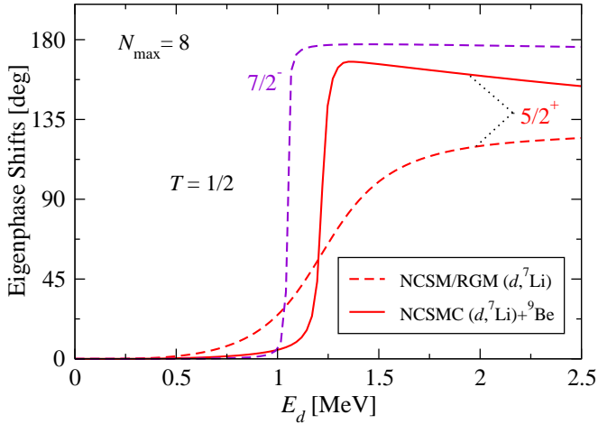
FIG. 5. Calculated d-{}^7\text{Li} eigenphase shifts in the J^\pi T = \frac{5}{2}^+ \frac{1}{2} and \frac{7}{2}^- \frac{1}{2} partial waves as function of the kinetic energy of the deuteron projectile in the laboratory system, resulting from (d,{}^7\text{Li}) NCSM/RGM (dashed lines) and (d,{}^7\text{Li})+{}^9\text{Be} NCSMC (solid line) calculations. The SRG- N^3\text{LO} NN potential with \Lambda = 2.02 \text{ fm}^{-1} , the N_{\text{max}} = 8 basis size, and the HO frequency of \hbar\Omega = 20 \text{ MeV} were used. For the \frac{7}{2}^- channel the NCSMC and NCSM/RGM eigenphase shifts are identical because the adopted set of {}^9\text{Be} eigenstates of Table III did not include states for this partial wave.
