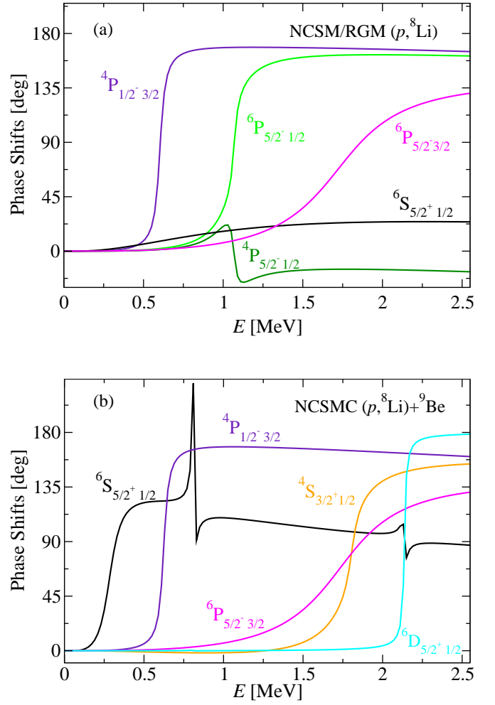
FIG. 4. Calculated p - {}^8\text{Li} elastic phase shifts within the (a) (p, {}^8\text{Li}) NCSM/RGM and (b) (p, {}^8\text{Li})+{}^9\text{Be} NCSMC bases as a function of the relative kinetic energy in the c.m. frame. The SRG- N^3\text{LO} NN potential with \Lambda = 2.02 \text{ fm}^{-1} , the N_{\text{max}} = 8 basis size, and the HO frequency of \hbar\Omega = 20 \text{ MeV} were used. The {}^9\text{Be} NCSM eigenstates used in the NCSMC calculation are specified in Table III.
