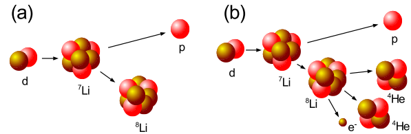
FIG. 1. {}^7\text{Li}(d,p){}^8\text{Li} reaction (a) as described in the present work, with the mass partitions in the entrance and exit channels modeled with cluster wave functions. The reaction as it is measured in experiment (b), where the detection apparatus can be based on 1) the counting of protons, 2) the beta decay of {}^8\text{Li} or 3) the yield of the {}^8\text{Be} (not shown in the figure) delayed alphas following the {}^8\text{Li} beta decay.
