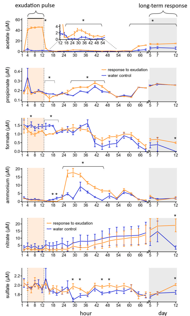
Fig. 2. Temporal dynamics of six soil metabolites ( \mu\text{M} ; acetate, propionate, formate, ammonium, nitrate, sulfate) in response to a 9-h long substrate pulse (orange) compared to a water control (blue). The time of the exudation pulse (4–12 h) is highlighted as an orange background and the long-term response (5–12 days) is highlighted as a grey background. The short-term response is depicted in hours and the long-term effects in days and are separated by an x-axis break at hour 72. Shown are the mean and standard error of the mean ( n = 5 ) of concentrations in collected dialysate. Acetate was part of the labile substrate pulse and its initial concentration in perfusate is depicted as a black horizontal line. The difference between the black horizontal line and the acetate measurements in dialysates illustrate the net transfer into the soil. Asterisks indicate that the response to labile substrate significantly differs from the water control. Detailed statistics are shown in Table 1. For net transfers and temporal dynamics of succinate, glucose and fructose, as well as temporal dynamics of citrate and oxalate (n.s.) see Fig. S4.
