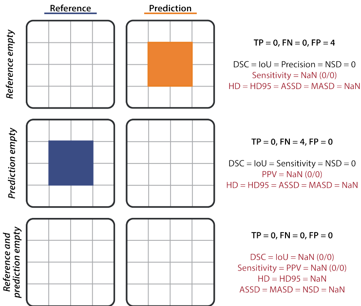
Extended Data Fig. SN 2.20. Effect of empty references or predictions when applying common metrics per image (here for semantic segmentation). Empty images lead to division by zero for many common metrics as the numbers of the TPs, FPs, FNPs turn zero. Used abbreviations: Average Symmetric Surface Distance (ASSD), Dice Similarity Coefficient (DSC), Hausdorff Distance (HD), Hausdorff Distance 95th Percentile (HD95), Intersection over Union (IoU), Mean Average Surface Distance (MASD), Not a Number (NaN), Normalized Surface Distance (NSD). This pitfall is also relevant for other boundary-based, overlap-based and counting metrics such as Boundary IoU, centerline Dice Similarity Coefficient (cIDice), F_{\beta} Score, Negative Predictive Value (NPV), Positive Predictive Value (PPV), Sensitivity, and Specificity.
