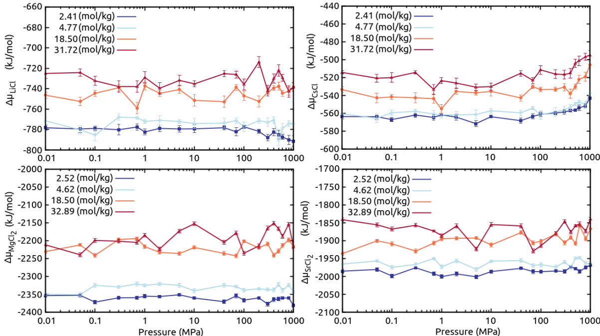
Figure 3: Chemical potential of ion exchange \Delta\mu_{C_nA_m}(P) as a function of pressure. Top-left: evolution of \Delta\mu_{LiCl}(P) . Top-right: evolution of \Delta\mu_{CsCl}(P) . Bottom-left: evolution of \Delta\mu_{MgCl_2}(P) . Bottom-right: evolution of \Delta\mu_{SrCl_2}(P) .
