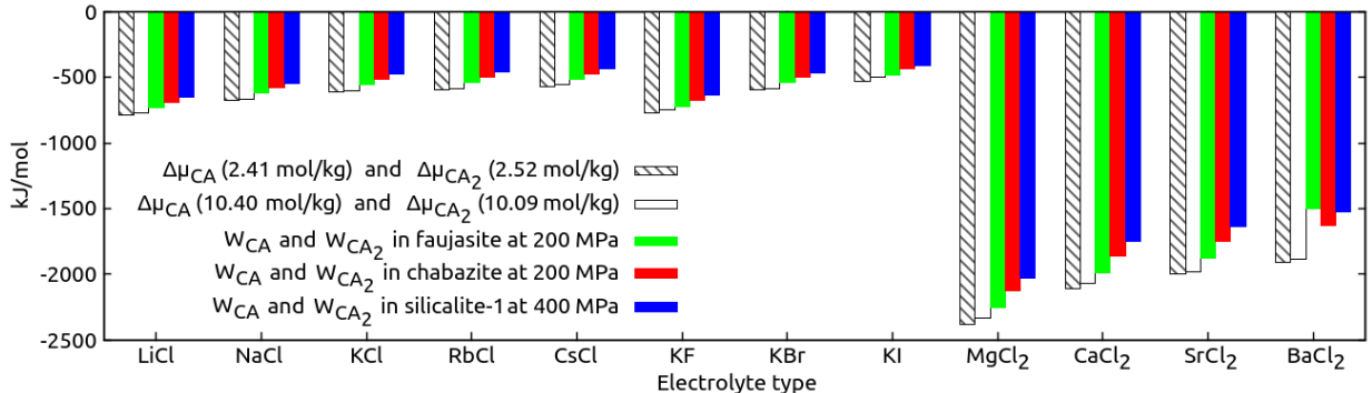
Figure 4: Histograms of the alchemical work W_{CA} for monovalent and W_{CA_2} for divalent-cation electrolytes associated to the intrusion of a single electrolyte unit in faujasite (green), chabazite (red) and silicalite-1 (blue). The chemical potential of ion exchange \Delta\mu_{CA} for monovalent and \Delta\mu_{CA_2} for divalent-cation electrolytes in the bulk for molalities of respectively 2.41, 10.40 and 2.52, 10.09 mol/kg are represented as dashed and white histograms.
