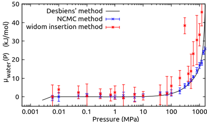
Figure 5: Chemical potential of TIP4P water estimated by three methods. Black curve : Desbiens' method. Blue points : Widom insertion method combined with NCMC move. Red points : Standard Widom insertion method.
