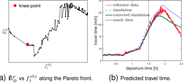
Fig. 7. SUMO-1 . Travel time prediction results for MOO approach.
