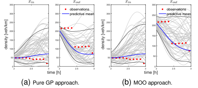
Fig. 8. SUMO-1 . Uncertainty quantification for pure GP and MOO approach.
