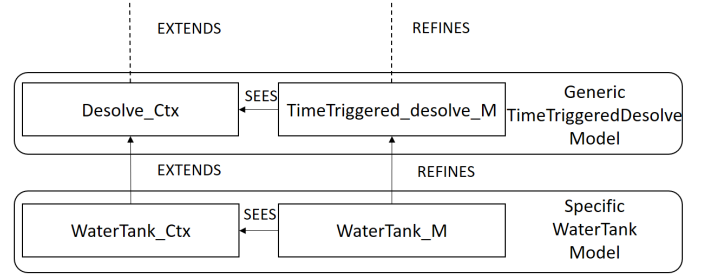
Fig. 12. Architecture of the EVENT-B model of the water tank system
