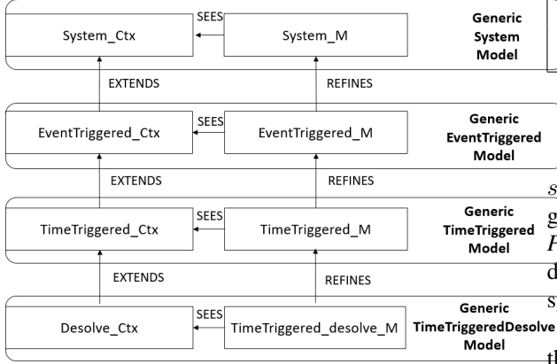
Fig. 2. Generic EVENT-B specification with the B_{desolve} function
