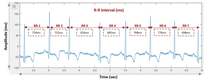
Fig. 6: Periods calculation of R-R interval.
