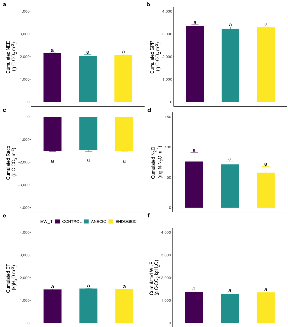
Figure 5. Cumulative fluxes of carbon, N_2O and water fluxes as affected by the earthworm treatments over the whole crop rotation. (a) NEE. (b) GPP. (c) Reco. (d) N_2O . (e) ET. (f) WUE. Data represent fluxes cumulated over 640 days \pm SEM of four replicates. Different letters above bars denote significant differences between means according to Tukey's HSD post-hoc test.
