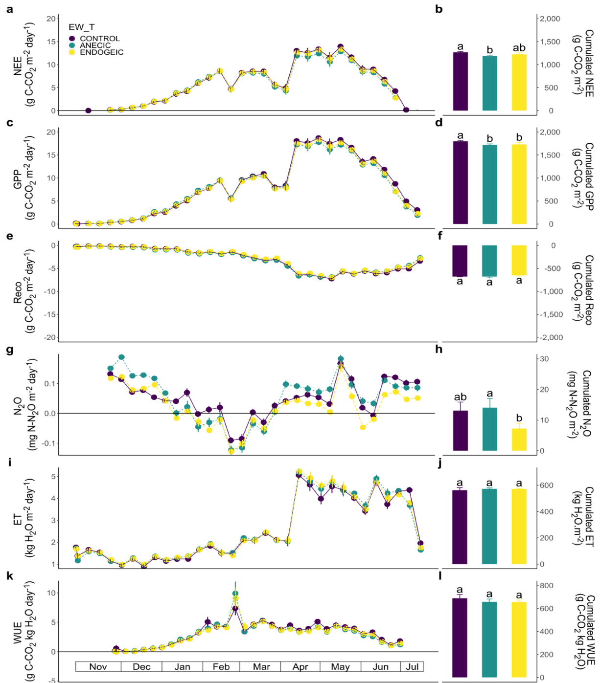
Figure 2. Weekly dynamics (left) and cumulative fluxes (right) of carbon, N_2O and water fluxes as affected by the earthworm treatments in the wheat crop. (a, b) NEE. (c, d) GPP. (e, f) Reco. (g, h) N_2O . (i, j) ET. (k, l) WUE. Data represent means \pm SEM of four replicates. Different letters above bars denote significant differences between means according to Tukey's HSD post-hoc test.
