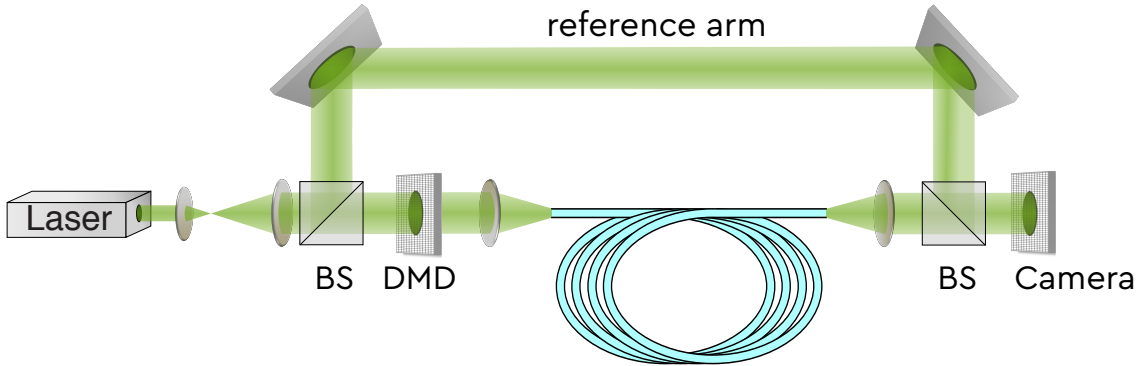
Figure 12: Measuring stability at the output of a multimode fiber. Schematic representation of the setup used to measure the phase fluctuations through a multimode fiber. An equivalent setup can be used with a scattering medium.
