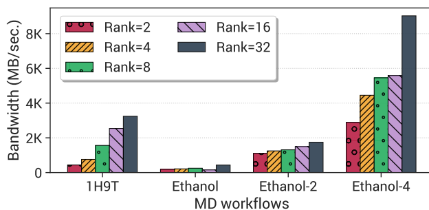
(b) VELOC checkpoint write bandwidth
