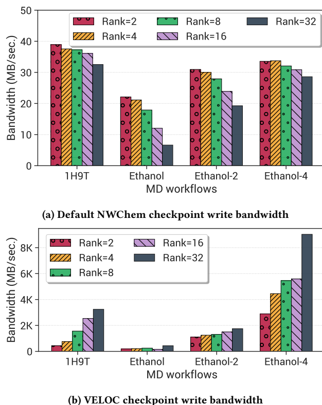
Figure 4: Analysis of checkpoint write bandwidth.
