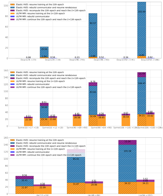
Figure 5: Costs (seconds) of recovering/reconfiguring workers when training the VGG-16 model in three scenarios: Scenario I: Dropping the failed process/node ("Down"); Scenario II: Remaining the original worker size by replacing the failed process/node with new process/node ("Same"); Scenario III: Automated doubling the worker size during the training ("Up"); scaling from 12 GPUs to utmost 192 GPUs
