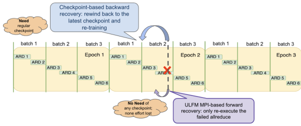
Figure 2: Backward recovery and proposed forward recovery based on ULMF MPI
