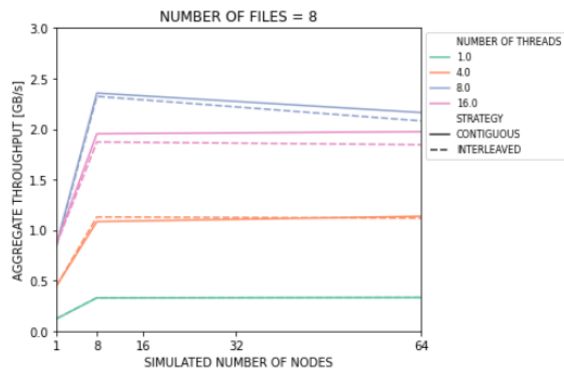
Fig. 3: Contiguous vs. interleaved aggregated throughput when number of files used for flushing = 8. Higher is better
