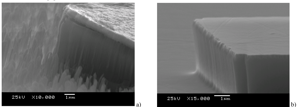
Fig. 2. 4H-SiC surfaces after RIE etching: (a) a rough SiC surface with grass aspect, (b) smooth SiC surface obtained with a Ni mask
