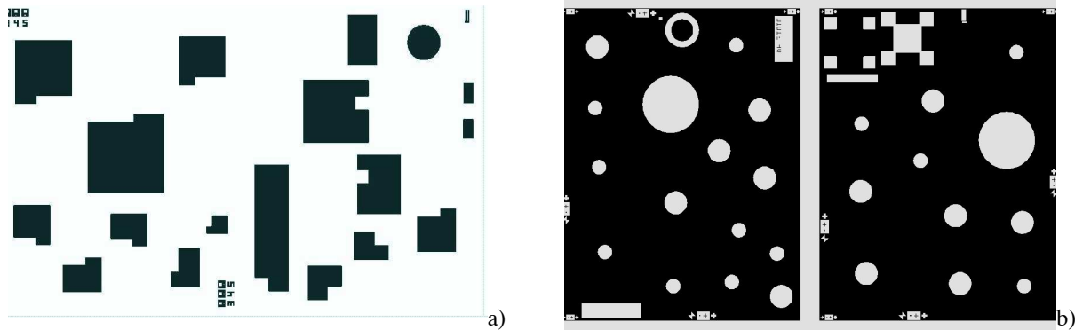
Fig. 4. Photomasks geometries used for the lithographic definition of the Ni (a), Si and C (b) mask structures. Field sizes are 6 by 10 \text{mm}^2 .
