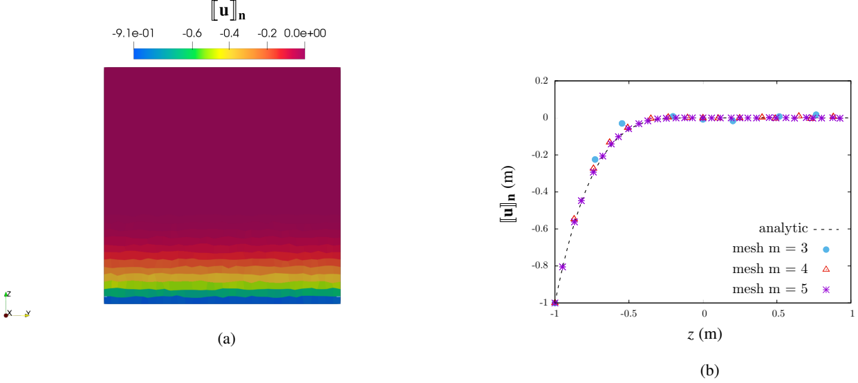
Figure 7. (a) Face-wise constant normal jump [[\mathbf{u}_{\mathcal{D}}]]_{\mathcal{D},\mathbf{n}} on \Gamma obtained on the hexahedral mesh with 2^{3m} cells, m = 5 . (b) Nodal normal jumps along the line x = y = 0 as a function of z both for the discrete solutions on the hexahedral meshes with 2^{3m} cells, m = 3, 4, 5 and for the continuous solution depending only on z . Test case of Section 4.1.1.
