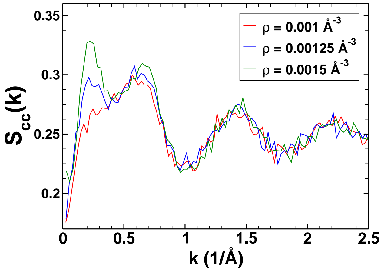
FIG. 4. Concentration-concentration structure factor for the Systems 1, 2 and 3.
