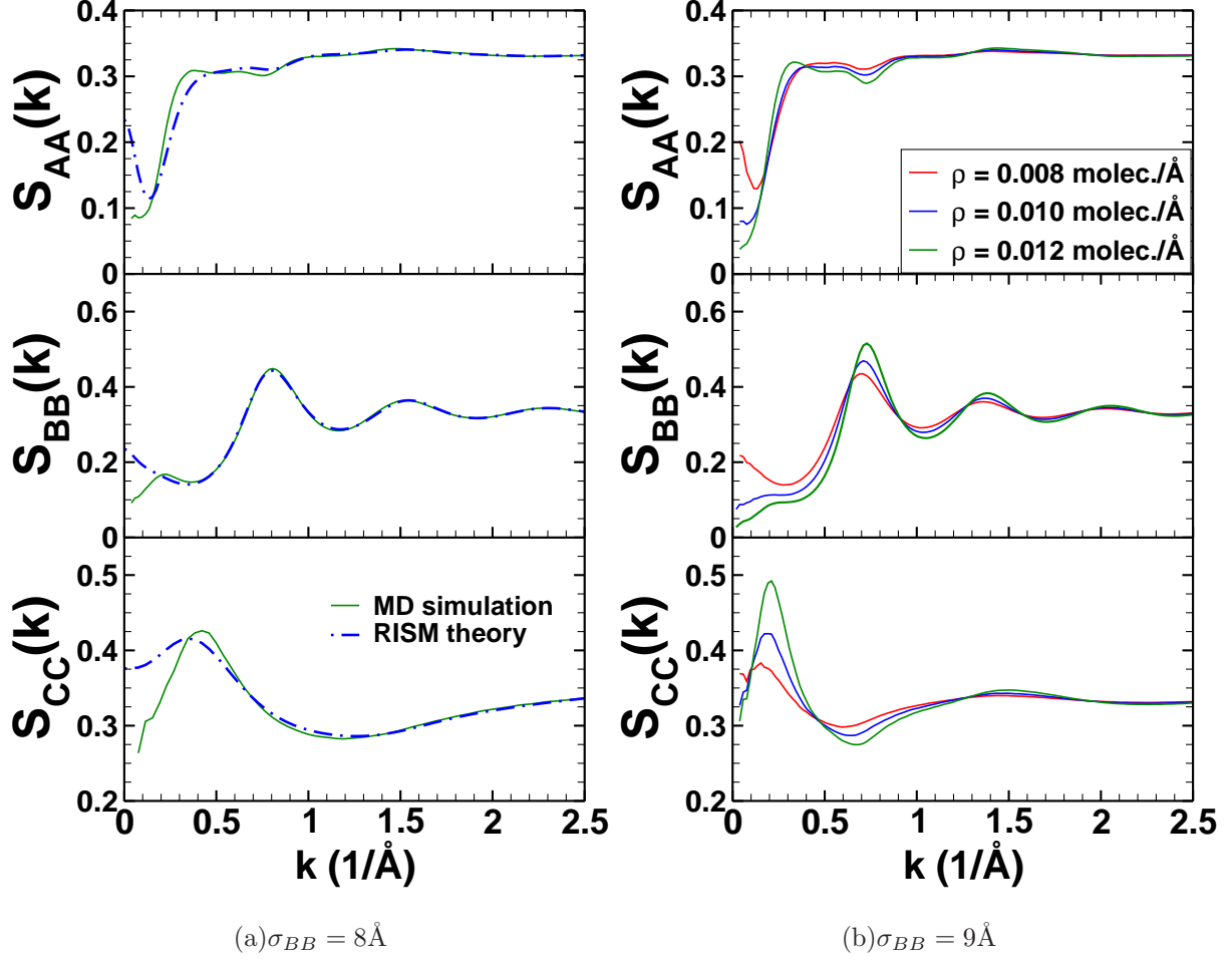
FIG. 3. The figures show the structure factors for A, B and C particles respectively. Column (a) corresponds to \sigma_{BB} = 8\text{\AA} for system 3 (theory vs. simulation) and column (b) presents the simulations results for systems 4 to 6 for \sigma_{BB} = 9\text{\AA} . Total density is indicated in the legend. Simulation results are represented by solid lines and dash-dotted curves correspond to integral equation calculations.
