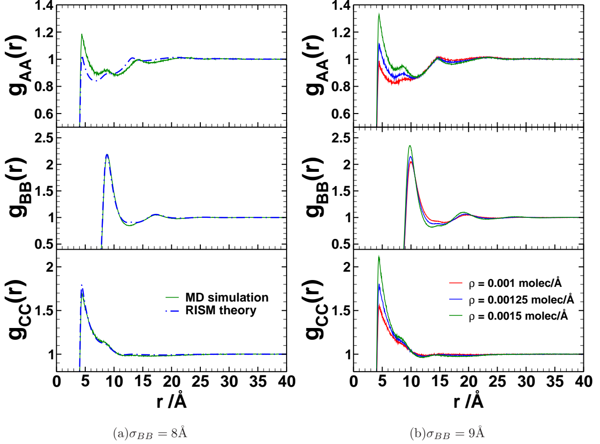
FIG. 2. The figures show the radial distribution functions for A, B and C particles respectively. Column (a) corresponds to \sigma_{BB} = 8\text{\AA} for system 3 (theory vs. simulation) and column (b) presents the simulation results for systems 4 to 6 for \sigma_{BB} = 9\text{\AA} . Total density is indicated in the legend. Simulation results are represented by solid lines and dash-dotted curves correspond to integral equation calculations.
