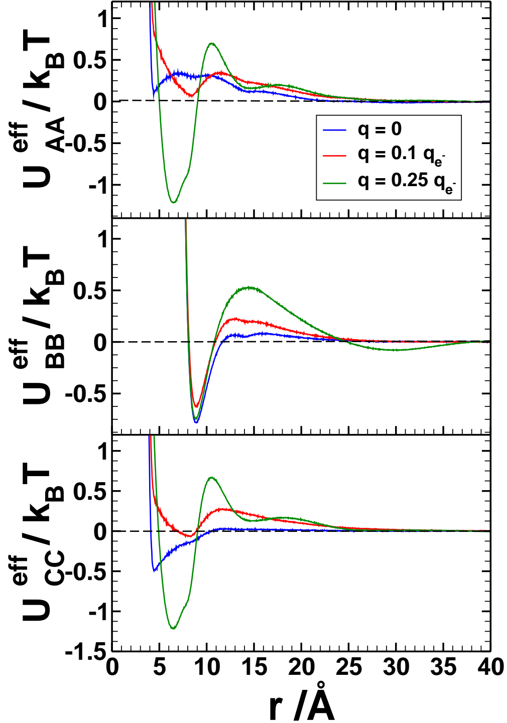
FIG. 11. Charge dependency of the effective potentials for A (top), B(middle) and C (bottom) particles. Charge magnitudes are specified in the legend. Values of r_{cl} correspond to the inflexion points of the effective potentials in their first minimum, i.e., r_{cl}(A - A) = 6 \text{ \AA} , r_{cl}(B - B) = 11 \text{ \AA} , r_{cl}(C - C) = 10 \text{ \AA}
