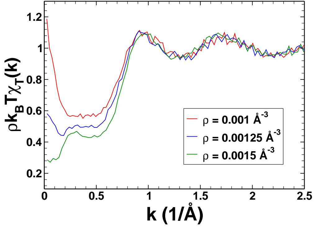
FIG. 5. Isothermal compressibility as a function of k for the Systems 1, 2 and 3.
