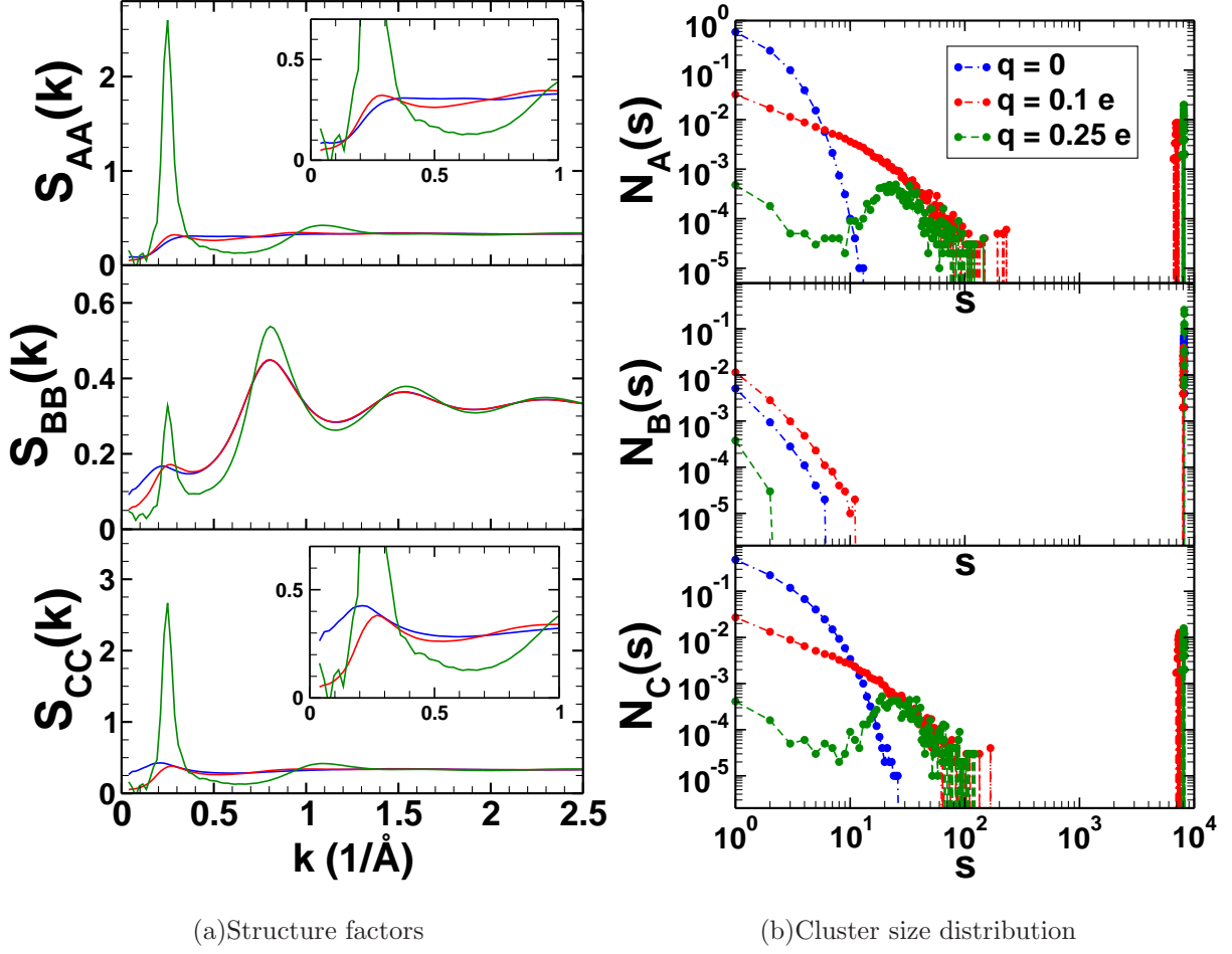
FIG. 10. (a) Charge dependence of the partial structure factors for A (top), B(middle) and C (bottom) particles (b) Charge dependence of the cluster size distribution. Charge magnitudes are specified in the legend.
