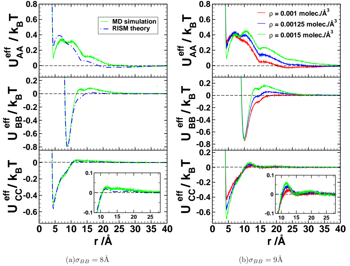
FIG. 6. Effective potentials for A, B and C particles respectively. Column (a) corresponds to \sigma_{BB} = 8\text{\AA} for system 3 (theory vs. simulation) and column (b) presents the simulations results for systems 4 to 6 for \sigma_{BB} = 9\text{\AA} . Total density is indicated in the legend. Simulation results are represented by solid lines and dash-dotted curves correspond to integral equation calculations.
