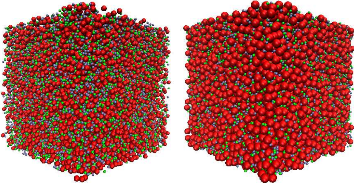
(a) \sigma_{BB} = 8\text{\AA}
