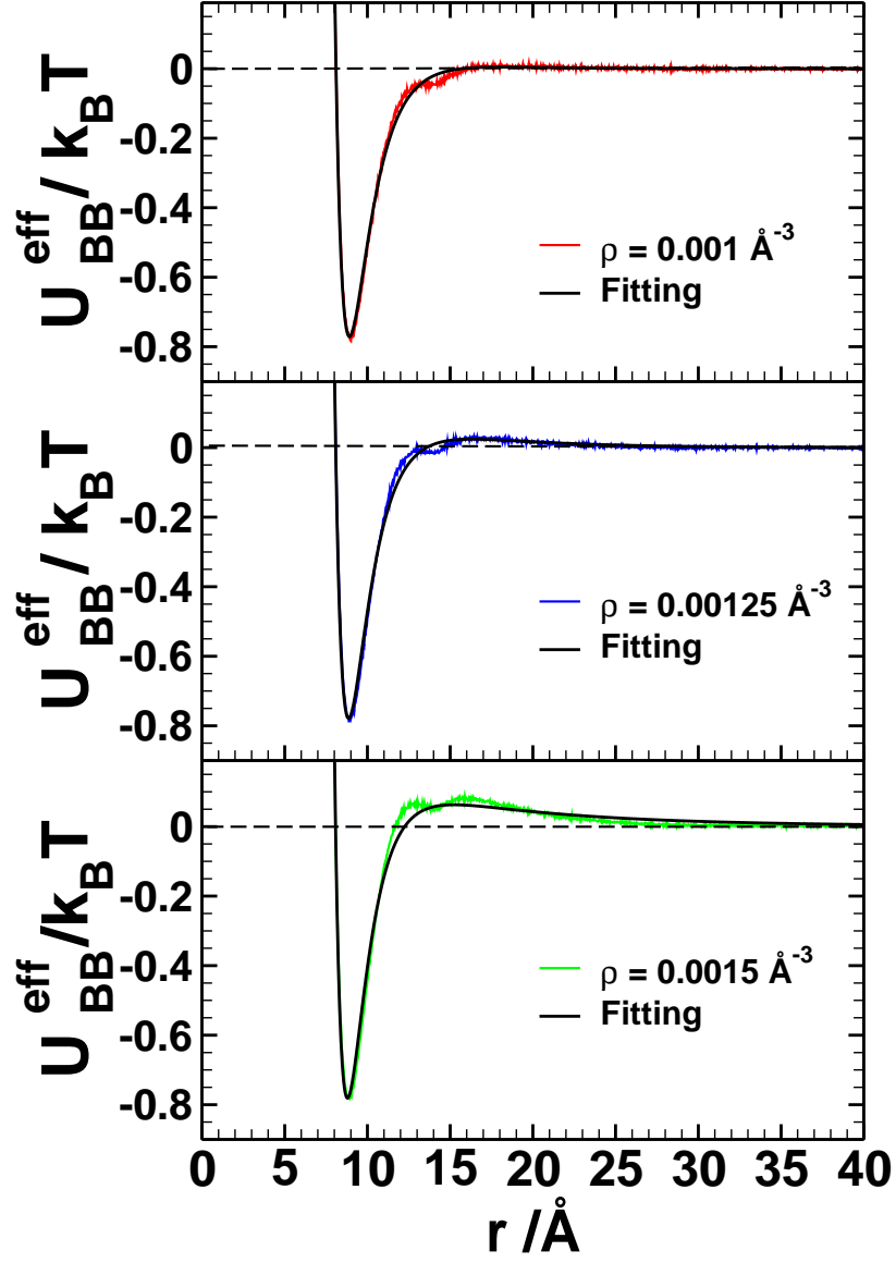
FIG. 7. B-B effective interaction for systems 1 to 3, fitted to a generalized LJ+Yukawa interaction
