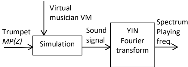
Figure 3. Block-diagram of the sound simulations
