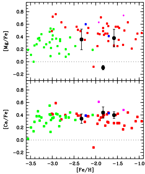
Fig. 4. [Mg/Fe] and [Ca/Fe] vs. [Fe/H] for the stars here analysed (black dots) in comparison to literature results: Cayrel et al. (green squares 2004), Fulbright (red squares 2000), Valentini et al. (pink squares 2019), Matas Pinto et al. (blue squares 2022).
