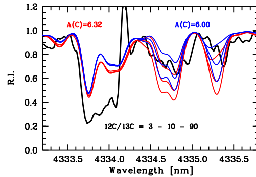
Fig. 6. TYC 5619-109-1 (solid black) in the G-band range. Over-plotted: synthetic spectra with two A(C) values and three ^{12}C/^{13}C ratios.
