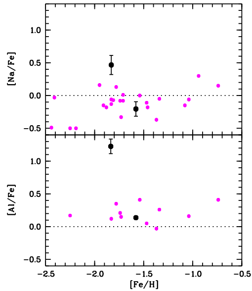
Fig. 5. [Na/Fe] and [Al/Fe] vs. [Fe/H] for two stars here analysed (TYC 5619-109-1 and TYC 9255-2088-1, black dots) in comparison results by Fulbright (2000).
