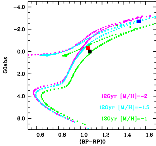
Fig. 3. The colour-magnitude diagram of the three stars here analysed as filled squares (red CD-37 8219, blue TYC 5619-1-9-1 and black TYC 9255-2088-1) compared to three PARSEC isochrones of 12 Gyr.
