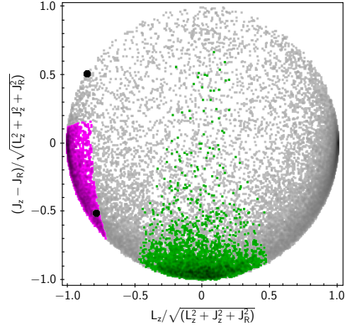
Fig. 1. The “action circle”. The two black symbols are the two high-speed stars of Matas Pinto et al. (2022). The background stars: gray dots the halo TO stars from Bonifacio et al. (2021); pink dots the stars of the Sequoia accretion event; green dots Gaia-Sausage-Enceladus stars. Star TYC 1193-1918-1 has actions compatible with the Sequoia structure, while TYC 622-742-1 is neither Sequoia nor GSE, thus a “halo” star.
