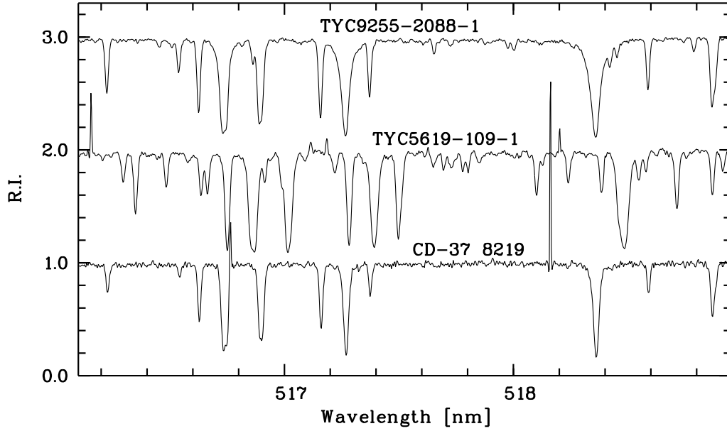
Fig. 2. The observed spectra in the range of the Mg b triplet.
