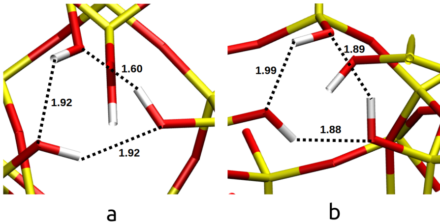
Figure 2: Silanol nest defects obtained from the local optimization procedure in silicalite-1 (a) and chabazite (b). The H atoms are in gray and the hydrogen bond lengths are labeled in Å.
