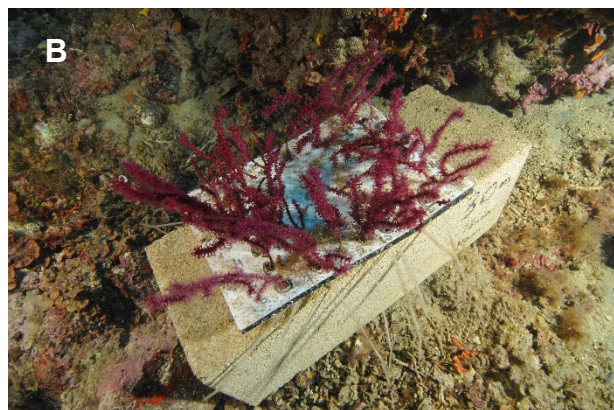
45 Fig. S2. Open quadrat used to characterize the size structure (50x50cm) (A) and Experi- 46 ment design for the transplantation of Paramuricea clavata colonies (samples of colonies 47 are fixed on a plastic plate and numbered) (B).
