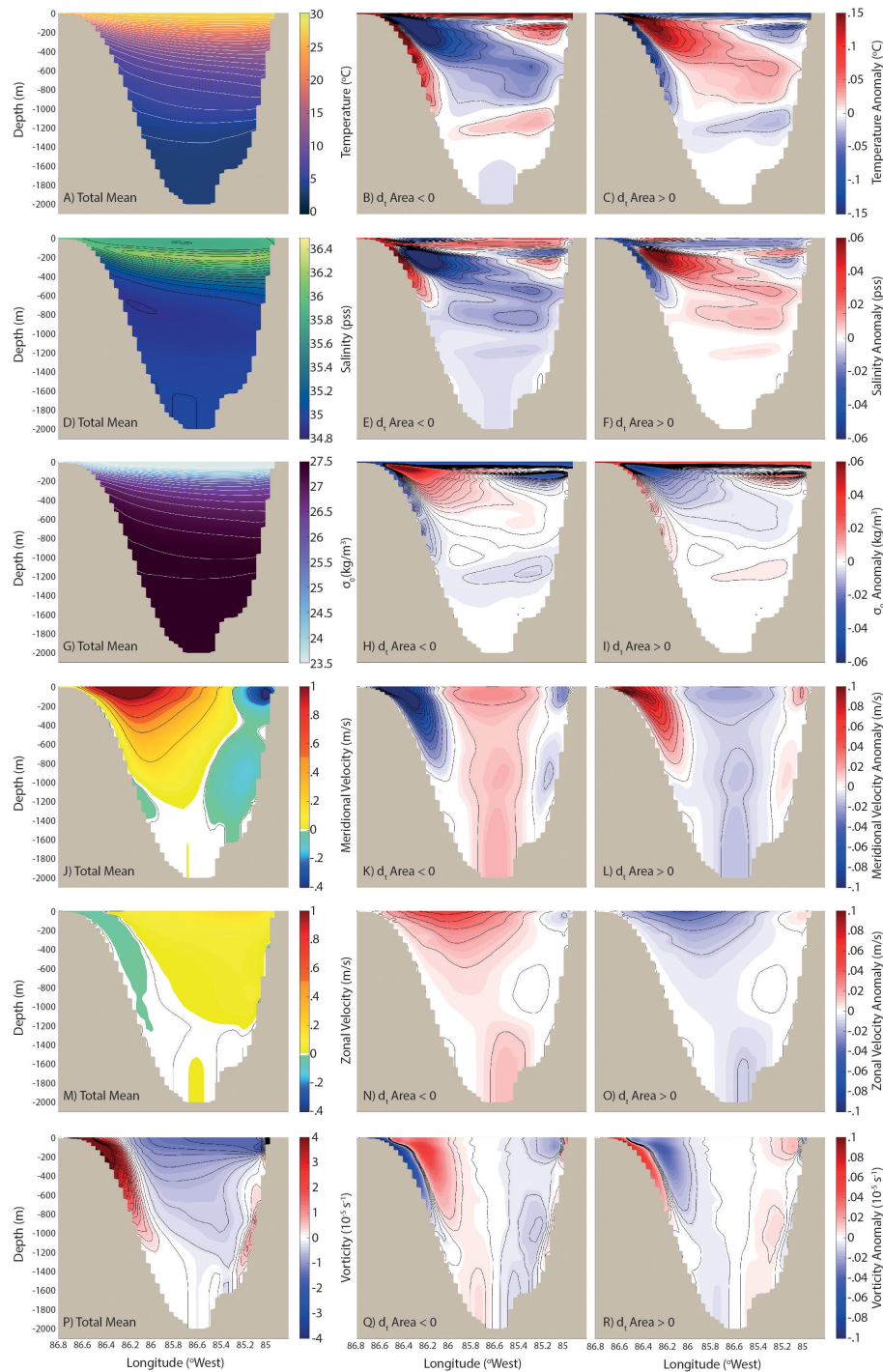
FIGURE 8 From the first to the last row, the fields of temperature, salinity, density, meridional, zonal velocities and vorticity respectively through the YC in the ClimBC simulation. The complete mean fields of these variables are shown in the first column and the associated mean anomalies when the LC “shrinks” and “grows” across the GoM are provided in the second and third columns respectively.
