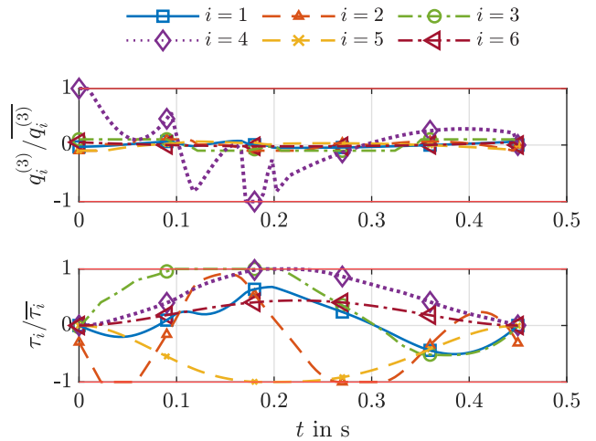
Fig. 7: Normalized joint jerk \ddot{\mathbf{q}} = \mathbf{q}^{(3)} and motor torques \tau of the Fanuc CRX10iA/L traversing from \mathbf{z}_a to \mathbf{z}_b .
