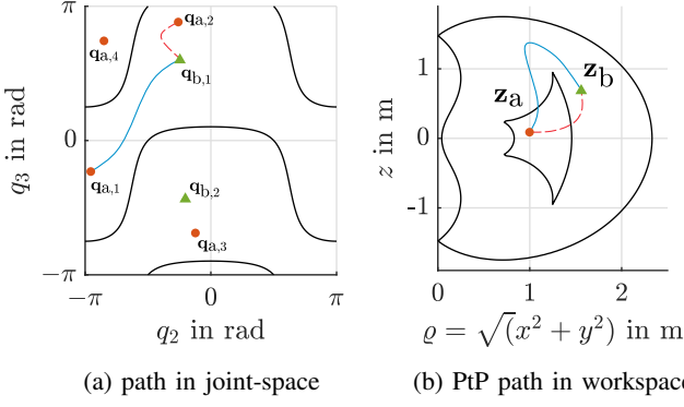
Fig. 1: joint-space a) and spherical cut of the workspace b) of a cuspidal 3R robot.
