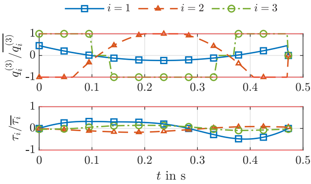
Fig. 4: Normalized joint jerk \ddot{\mathbf{q}} = \mathbf{q}^{(3)} and motor torques \tau of the 3R manipulator traversing from \mathbf{z}_a to \mathbf{z}_b .
