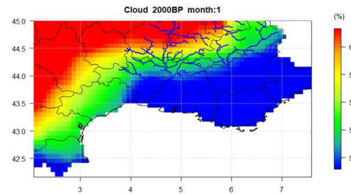
Cloud cover
