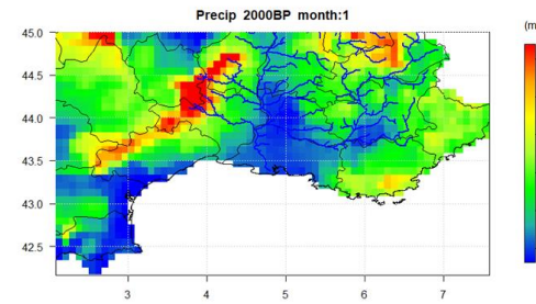
Precipitations
