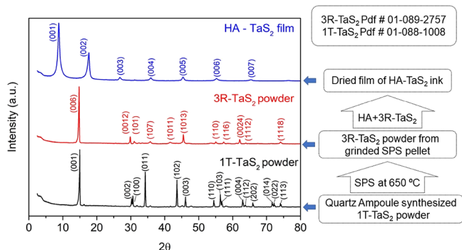
Figure 1. XRD pattern for the intermediate and products. The material that is synthesized in the ampoule shows the 1T-TaS 2 ; after post-treatment, the 3R-TaS 2 and hexylamine-intercalated 3R-TaS 2 (HA-TaS 2 ) were successfully formed.
