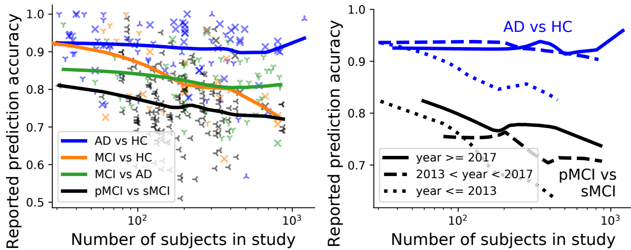
Fig. 1. Larger brain-imaging datasets are not enough for better machine-learning diagnosis of Alzheimer’s. A meta-analysis across 6 review papers, covering more than 500 individual publications. The problem is typically formulated as distinguishing Alzheimer’s disease (AD), healthy control (HC), and mild cognitive impairment (MCI), which can signal the onset of Alzheimer’s. Distinguishing progressive mild cognitive impairment (pMCI) from stable mild cognitive impairment (sMCI) is the most relevant machine-learning task from the clinical standpoint. Left: Reported prediction accuracy as a function of the number of subjects in a study. Right: Same plot distinguishing studies published in different years.
